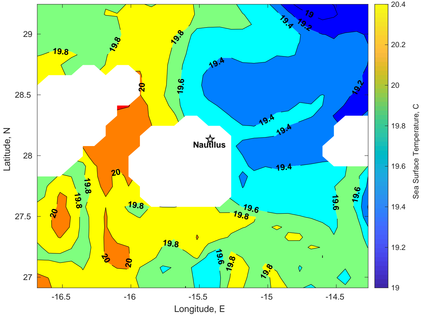
SST for Nautilus at 10-Mar-2025 00:00:00
