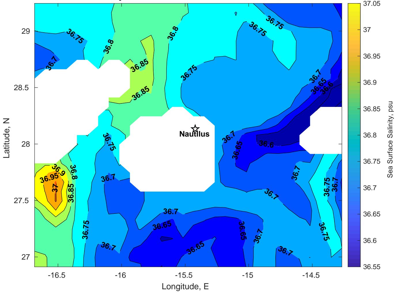
Surface Salinity for Nautilus at 10-Mar-2025 00:00:00
