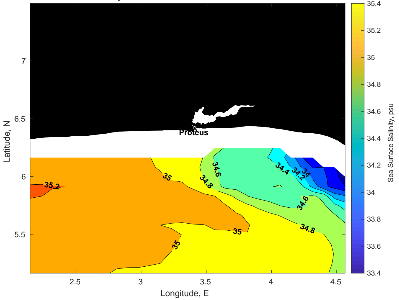
Surface Salinity for Proteus at 10-Mar-2025 00:00:00
