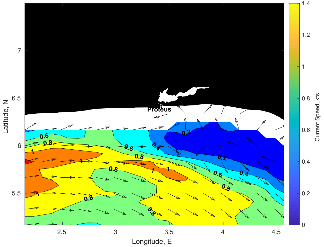
Surface Currents for Proteus at 10-Mar-2025 00:00:00
