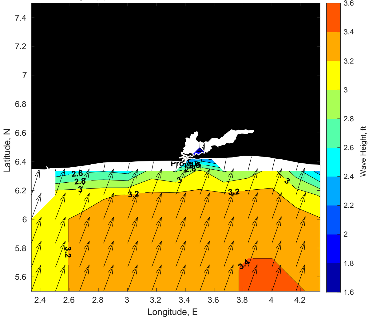
Wave Height (ft) for Proteus at 11-Mar-2025 09:00:00
