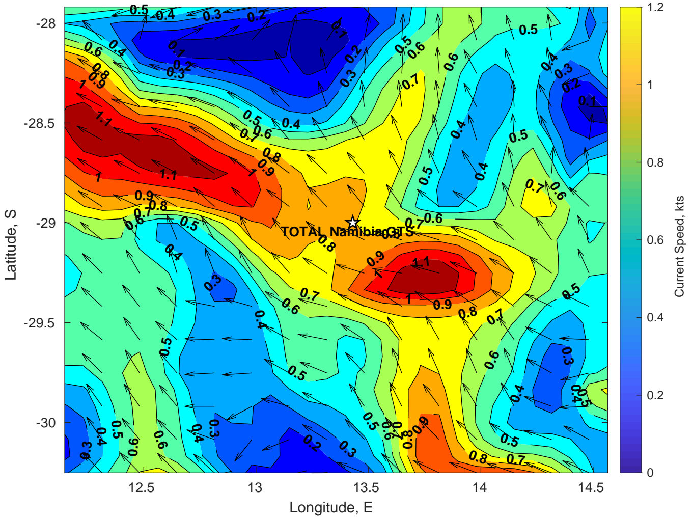
Surface Currents for TOTAL Namibia GTS at 10-Mar-2025 00:00:00
