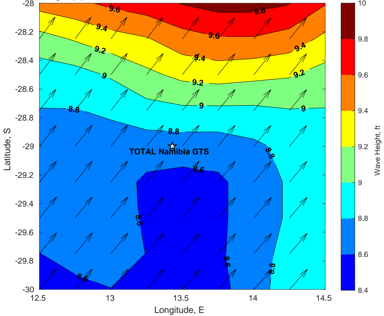
Wave Height (ft) for TOTAL Namibia GTS at 11-Mar-2025 09:00:00
