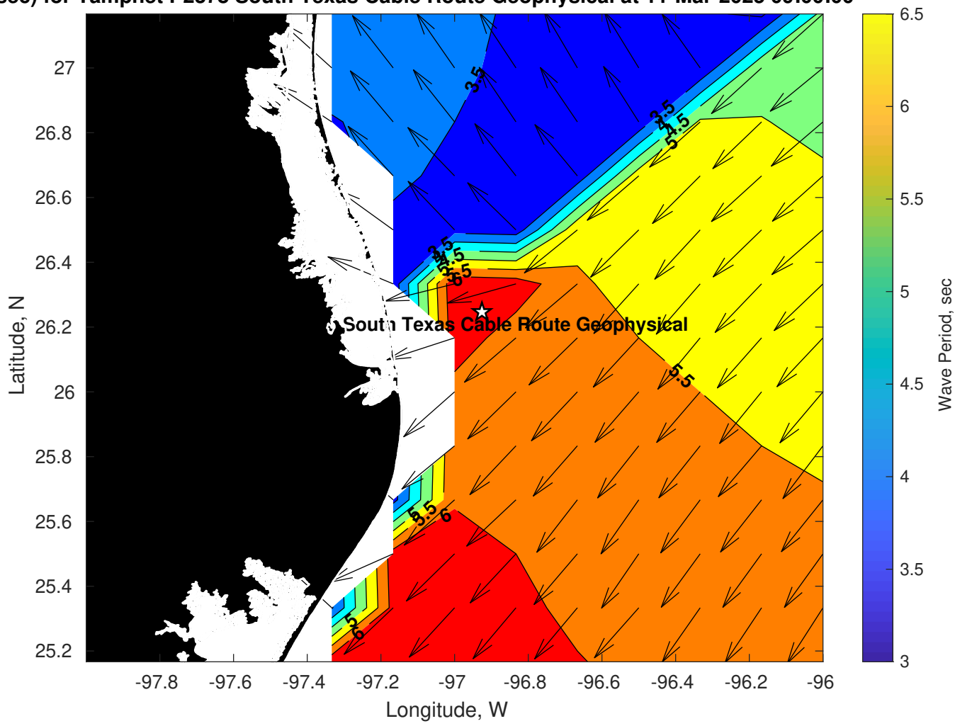
Period (sec) for Tampnet P2378 South Texas Cable Route Geophysical at 11-Mar-2025 09:00:00
