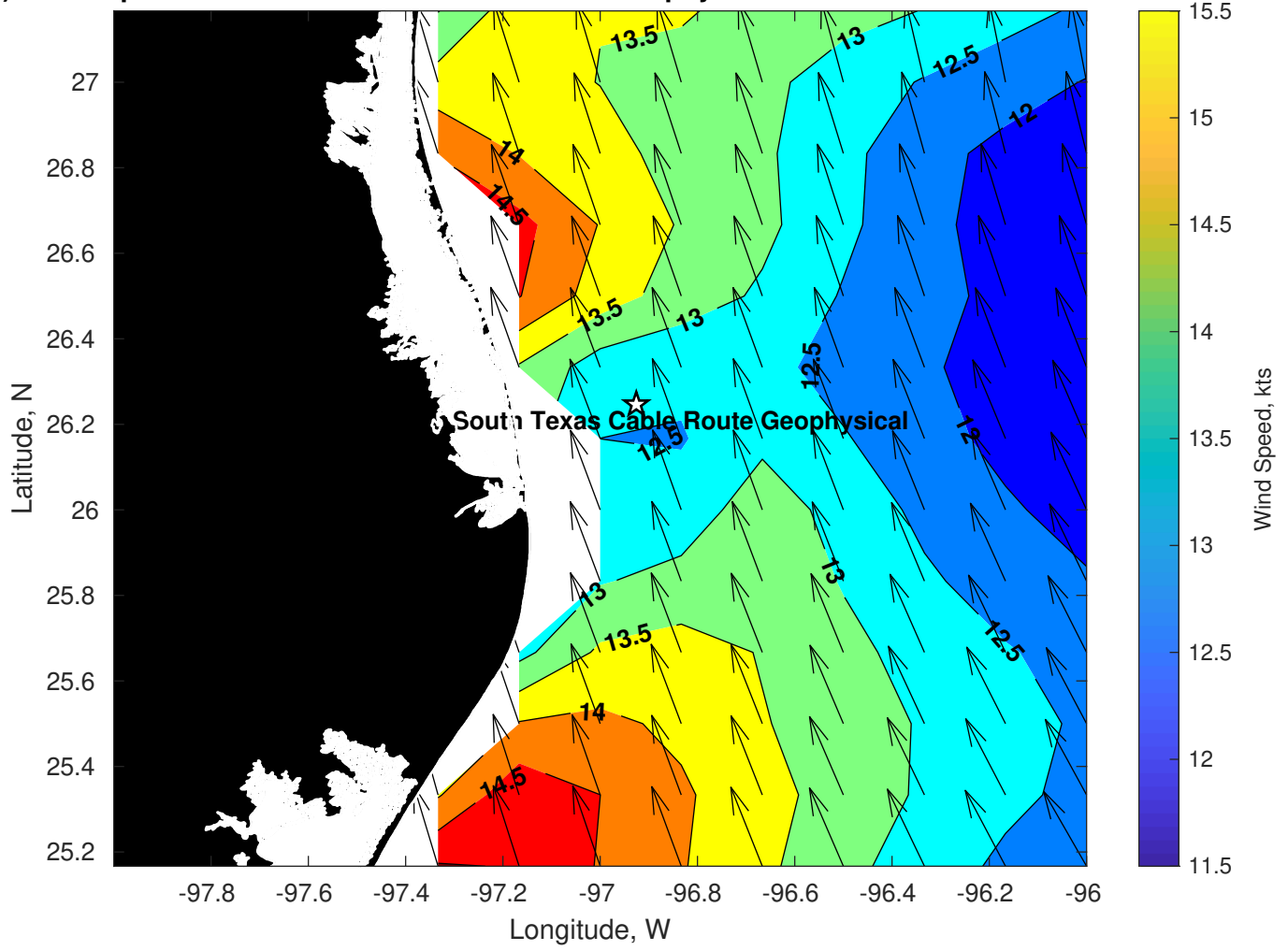
Winds (kts) for Tampnet P2378 South Texas Cable Route Geophysical at 11-Mar-2025 09:00:00
