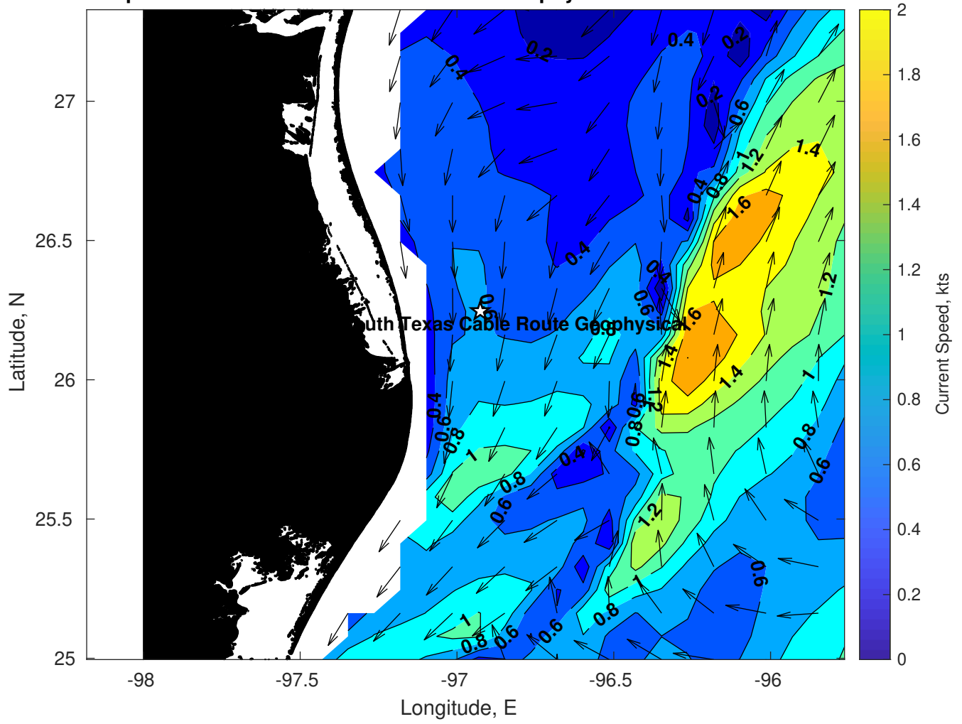
Surface Currents for Tampnet P2378 South Texas Cable Route Geophysical at 10-Mar-2025 00:00:00
