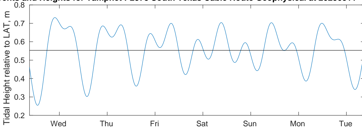
Tidal Currents and Heights for Tampnet P2378 South Texas Cable Route Geophysical at 20250311
