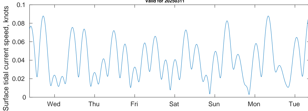
Tidal Currents and Heights for Tampnet P2378 South Texas Cable Route Geophysical at 20250311
