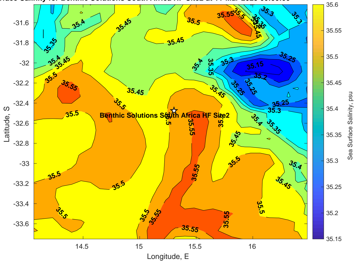
Surface Salinity for Benthic Solutions South Africa HF Site2 at 11-Mar-2025 00:00:00
