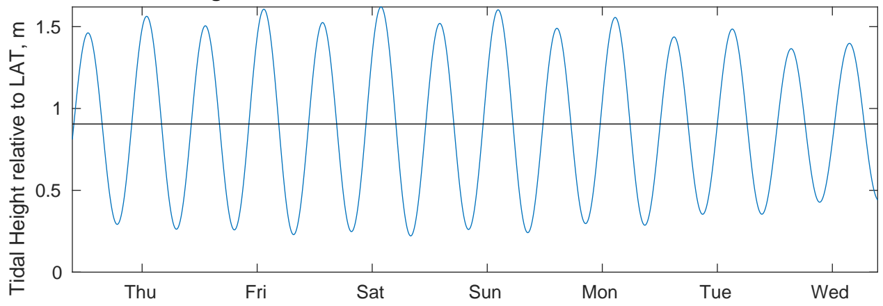
Tidal Currents and Heights for Benthic Solutions South Africa HF Site2 at 20250312
