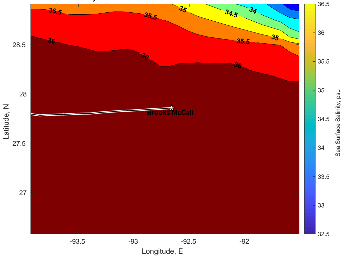
Surface Salinity for Brooks McCall at 11-Mar-2025 00:00:00
