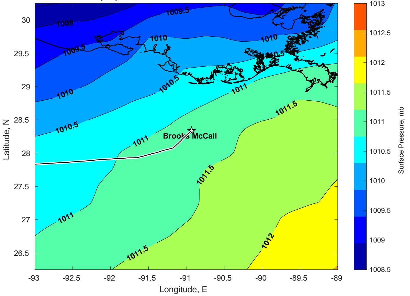
Surface Pressure (mb) for Brooks McCall at 14-Mar-2025 00:00:00
