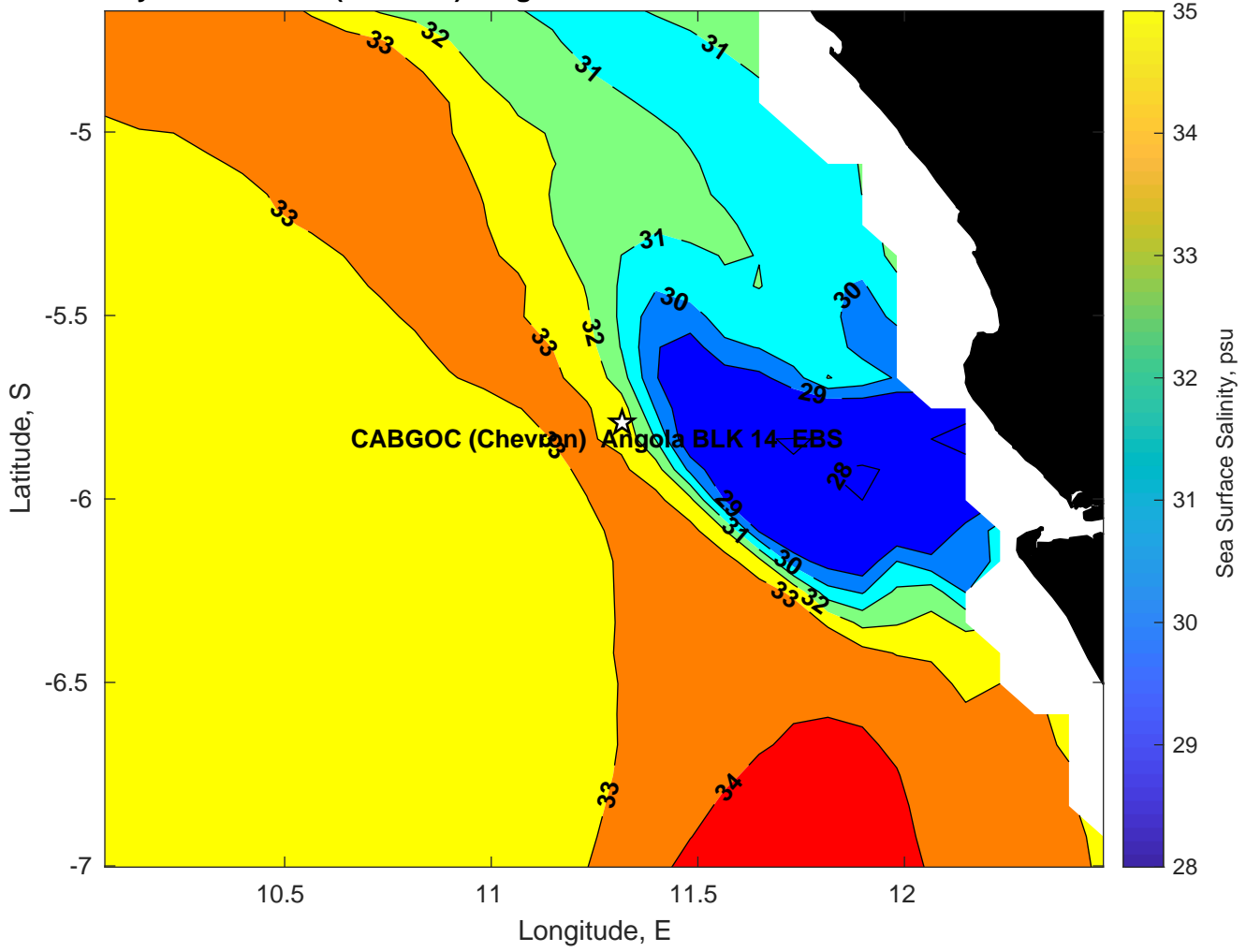
Surface Salinity for CABGOC (Chevron) Angola BLK 14 EBS at 11-Mar-2025 00:00:00
