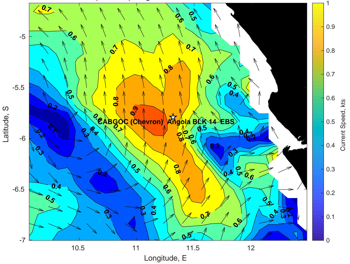
Surface Currents for CABGOC (Chevron) Angola BLK 14 EBS at 11-Mar-2025 00:00:00
