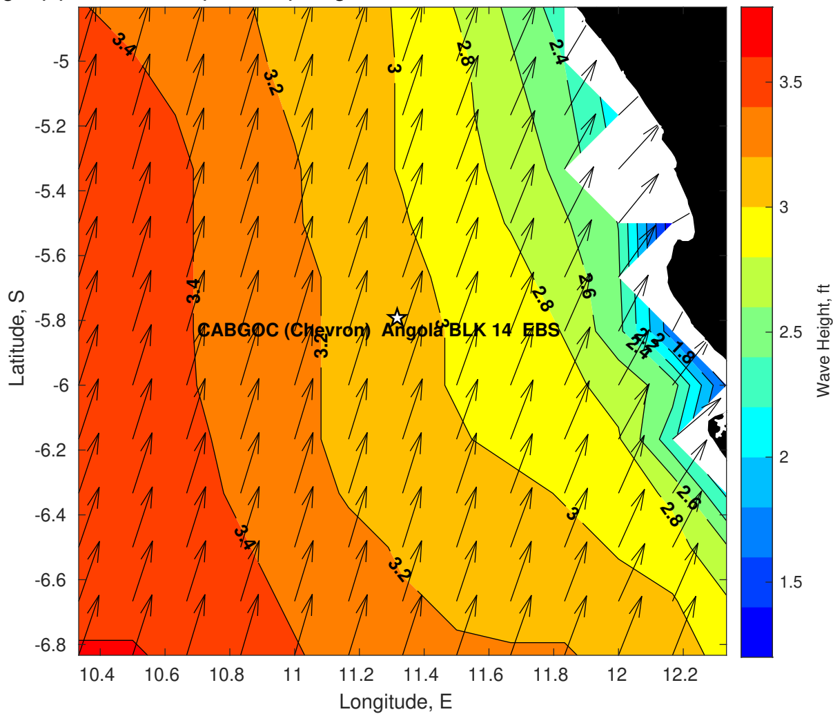
Wave Height (ft) for CABGOC (Chevron) Angola BLK 14 EBS at 12-Mar-2025 09:00:00
