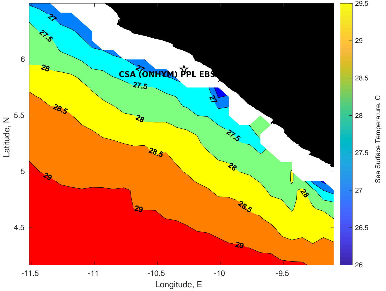
SST for CSA (ONHYM) PPL EBS - Liberia at 11-Mar-2025 00:00:00
