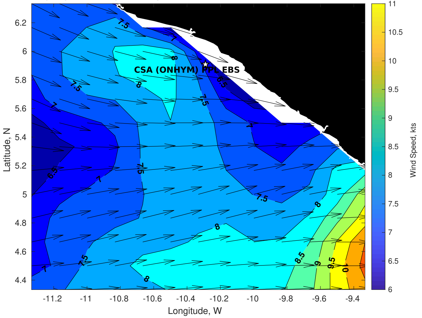
Winds (kts) for CSA (ONHYM) PPL EBS - Liberia at 12-Mar-2025 09:00:00
