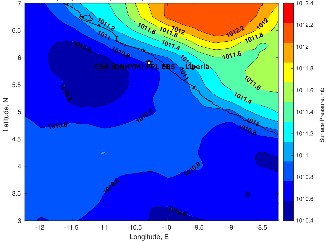
Surface Pressure (mb) for CSA (ONHYM) PPL EBS - Liberia at 14-Mar-2025 00:00:00
