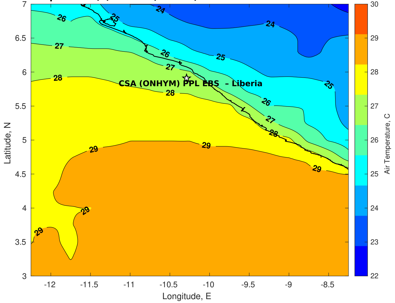
Air Temperature (C) for CSA (ONHYM) PPL EBS - Liberia at 12-Mar-2025
