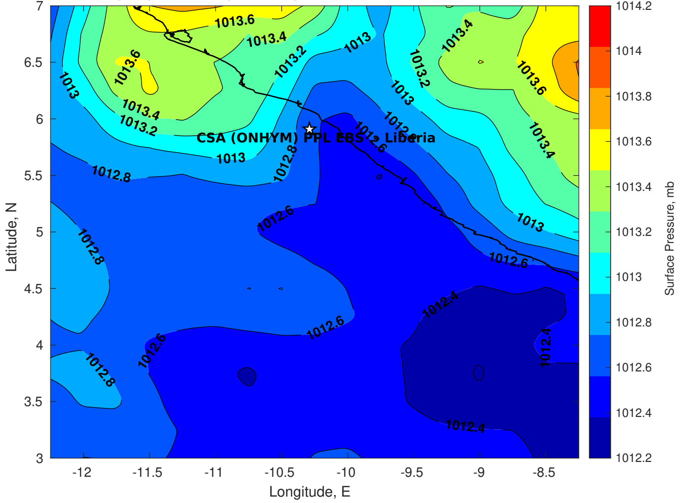
Surface Pressure (mb) for CSA (ONHYM) PPL EBS - Liberia at 12-Mar-2025 00:00:00
