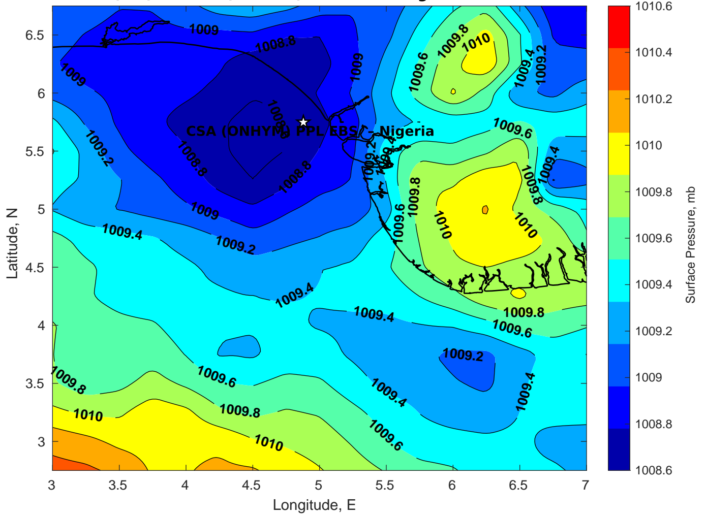
Surface Pressure (mb) for CSA (ONHYM) PPL EBS - Nigeria at 12-Mar-2025 00:00:00
