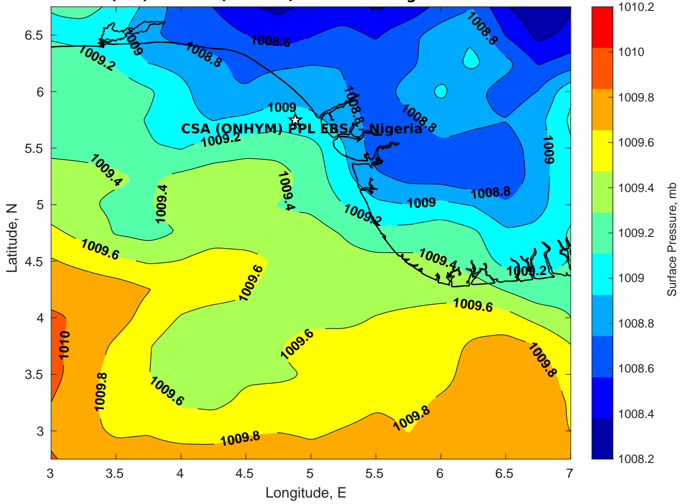
Surface Pressure (mb) for CSA (ONHYM) PPL EBS - Nigeria at 14-Mar-2025 00:00:00
