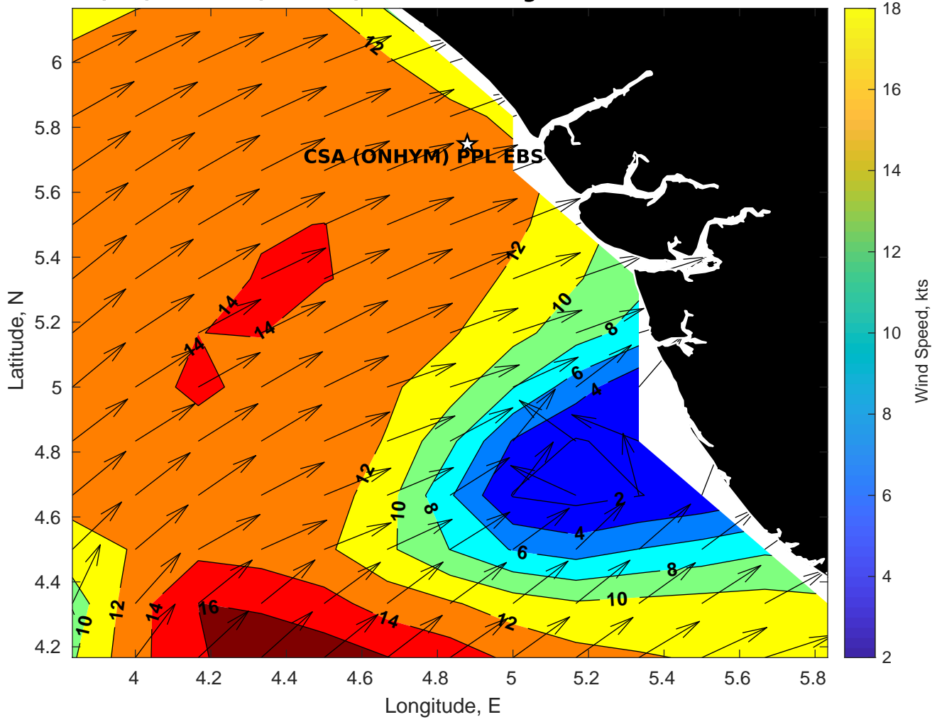
Winds (kts) for CSA (ONHYM) PPL EBS - Nigeria at 12-Mar-2025 09:00:00
