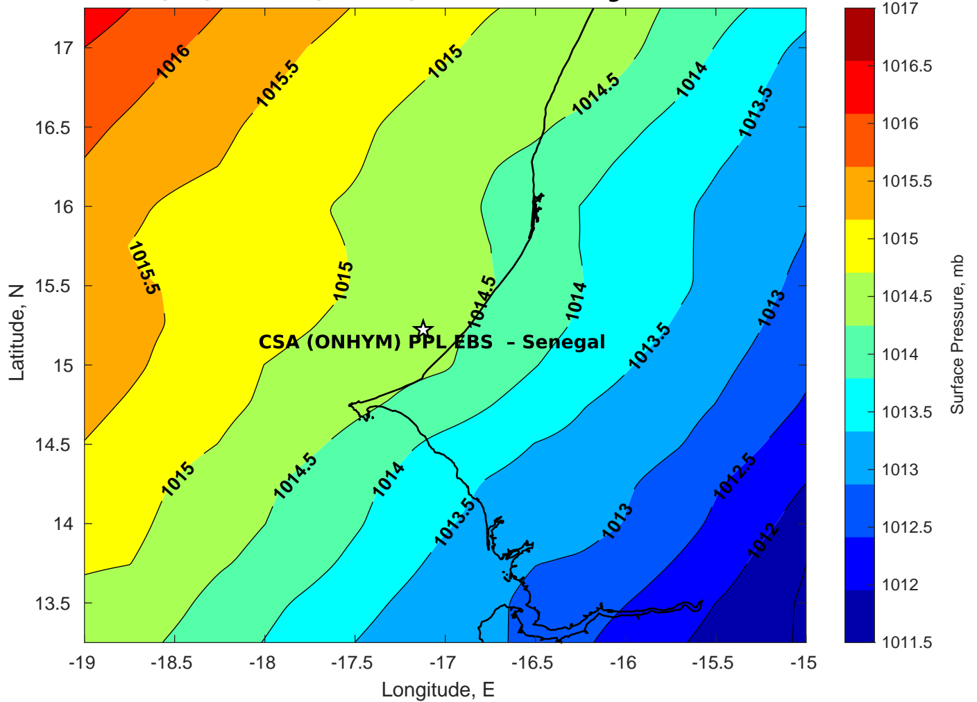
Surface Pressure (mb) for CSA (ONHYM) PPL EBS - Senegal at 12-Mar-2025 00:00:00
