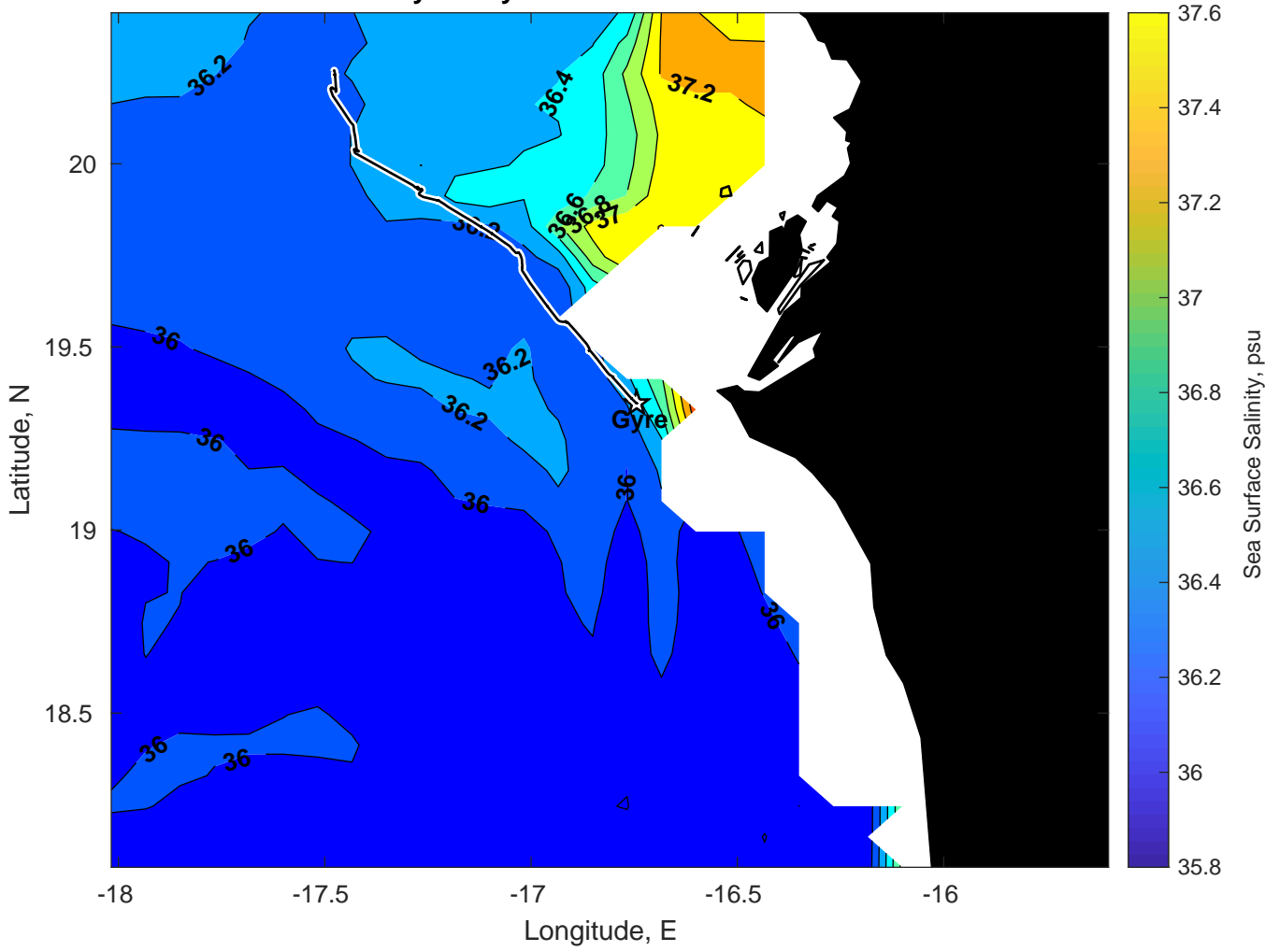
Surface Salinity for Gyre at 11-Mar-2025 00:00:00
