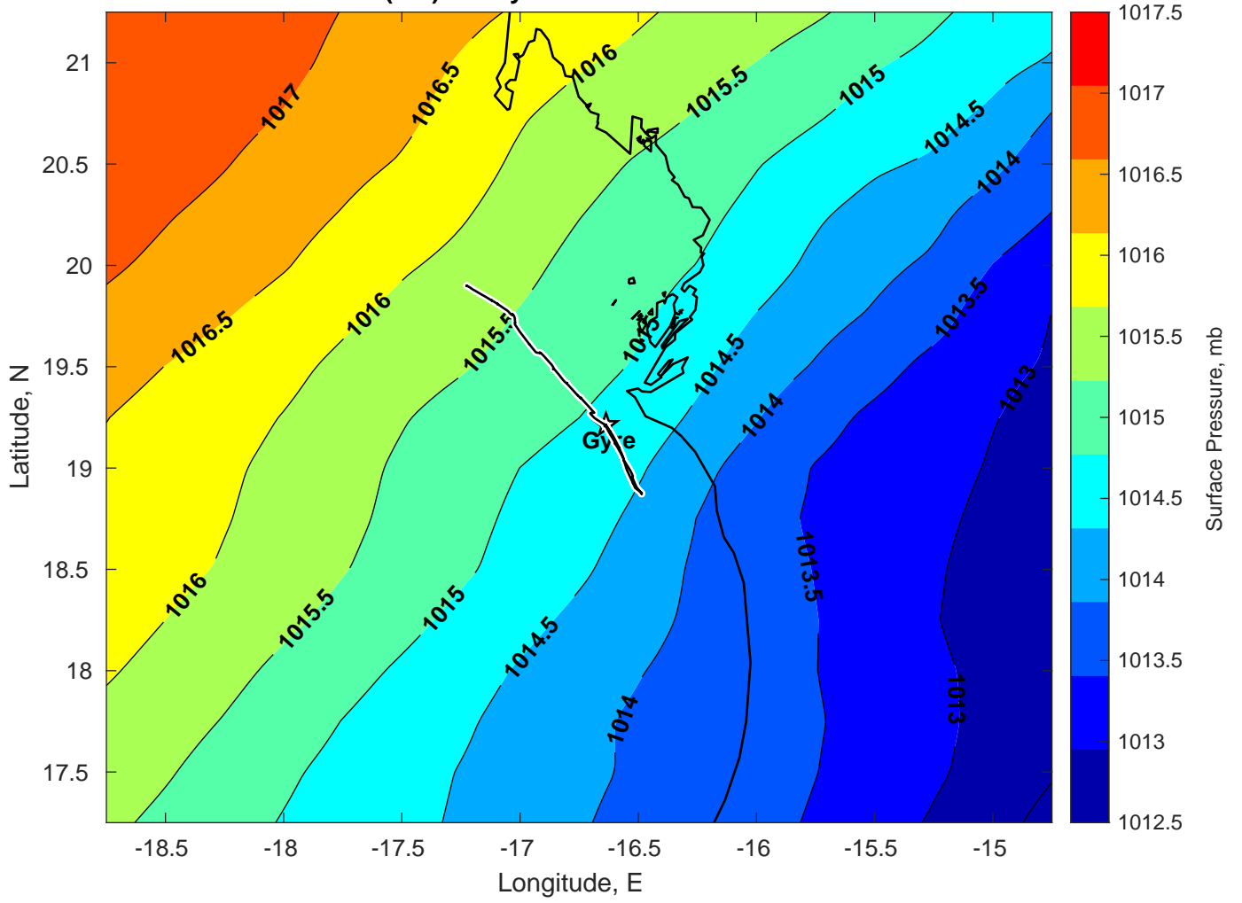
Surface Pressure (mb) for Gyre at 13-Mar-2025 00:00:00
