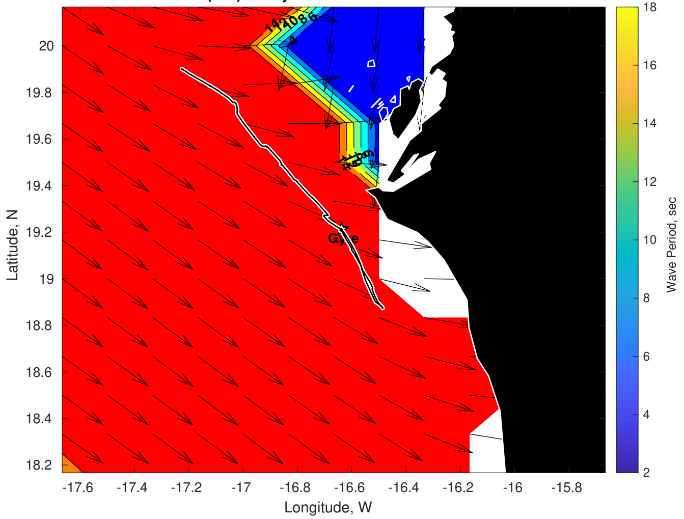
Wave Period (sec) for Gyre at 12-Mar-2025 09:00:00
