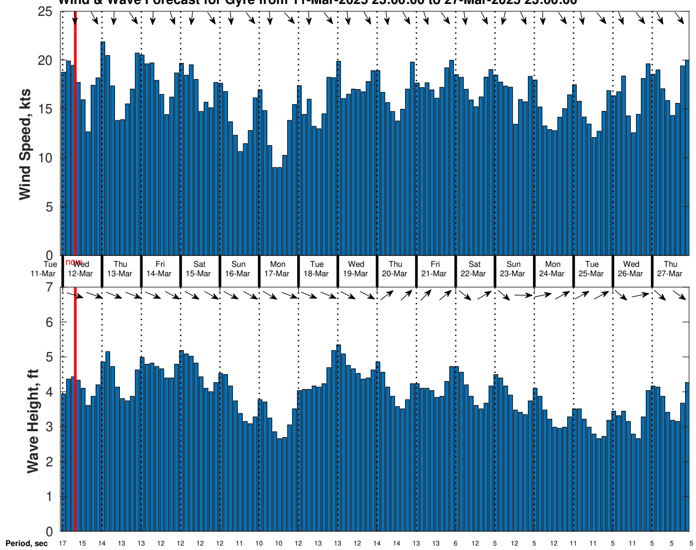
Wind & Wave Forecast for Gyre from 11-Mar-2025 23:00:00 to 27-Mar-2025 23:00:00
