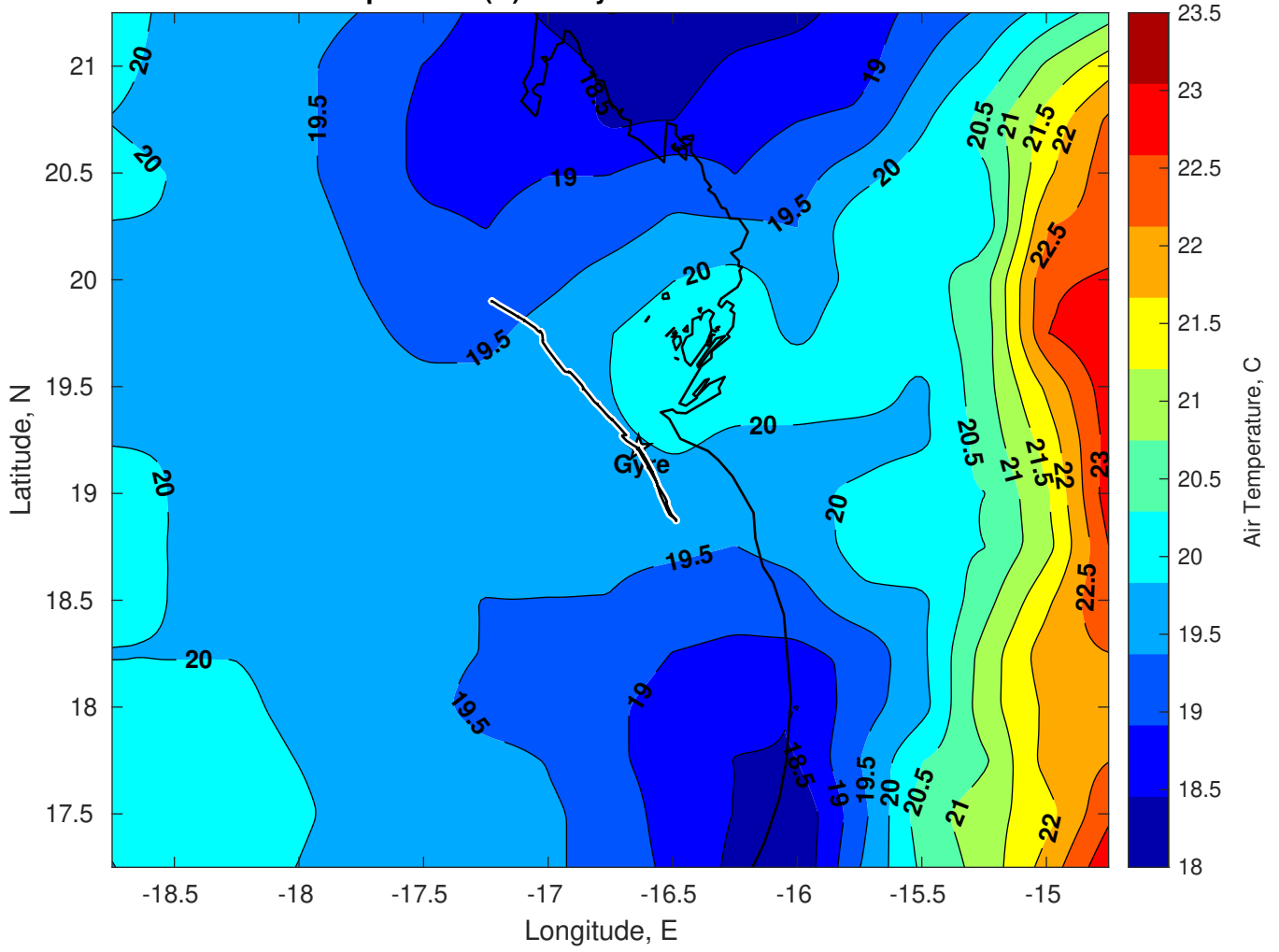
Air Temperature (C) for Gyre at 12-Mar-2025
