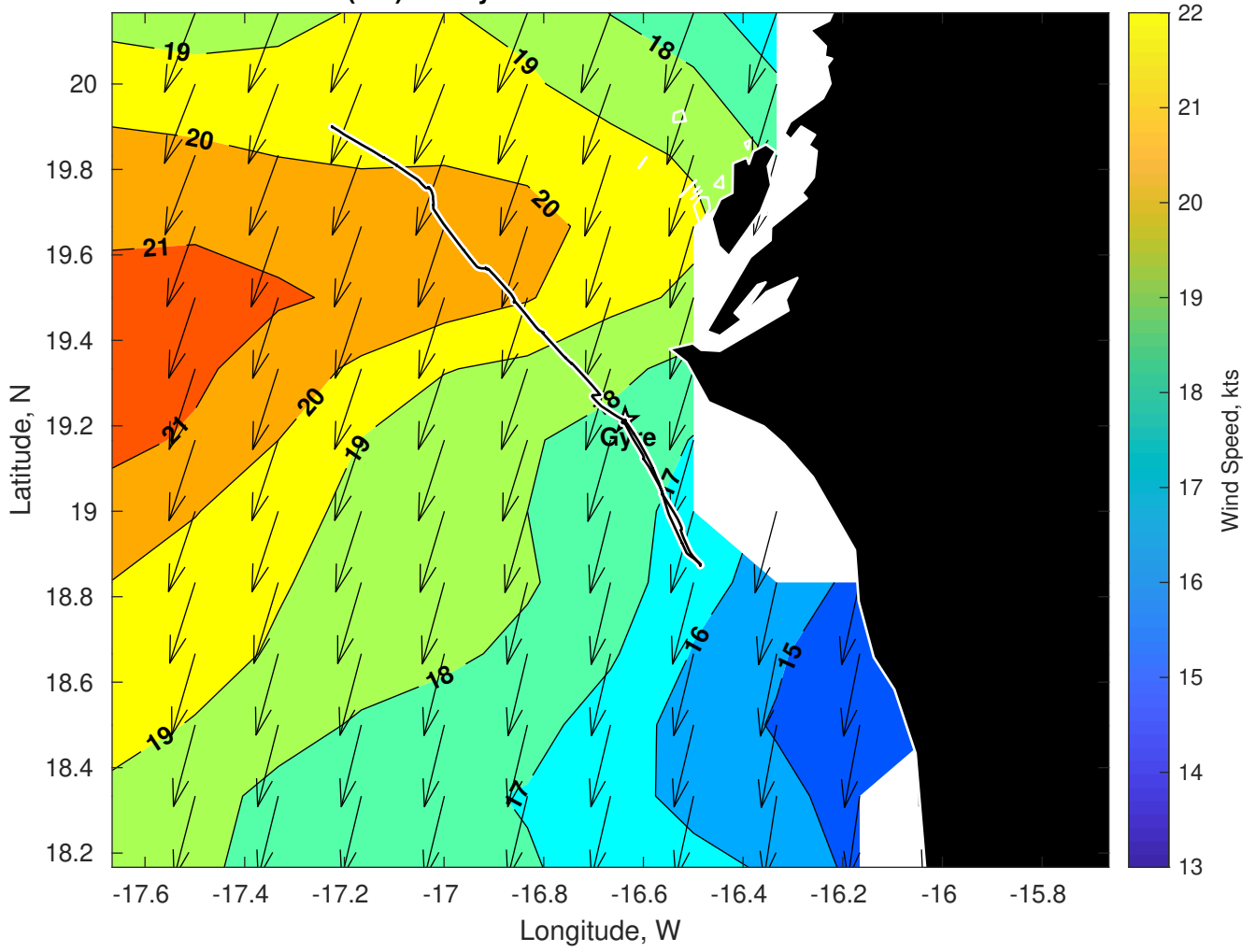
Winds (kts) for Gyre at 12-Mar-2025 09:00:00
