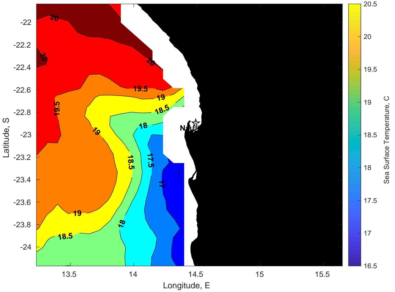
SST for Nautilus at 11-Mar-2025 00:00:00
