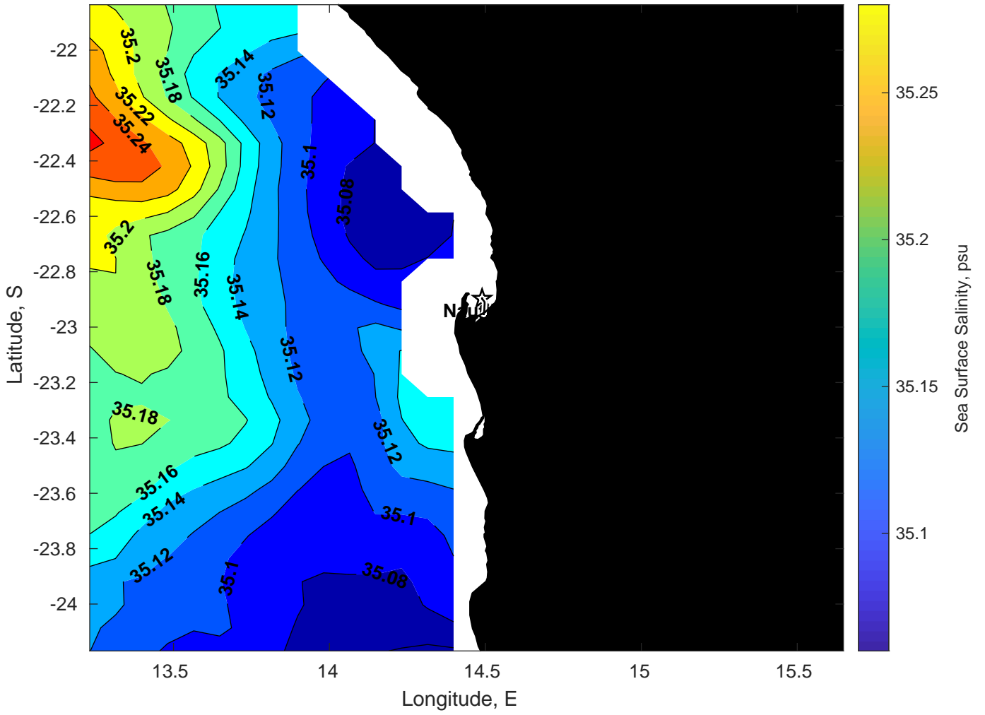
Surface Salinity for Nautilus at 11-Mar-2025 00:00:00
