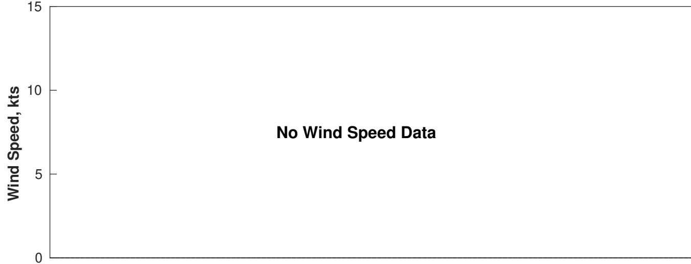
Wind & Wave Forecast for Nautilus from 12-Mar-2025 02:00:00 to 28-Mar-2025 02:00:00
