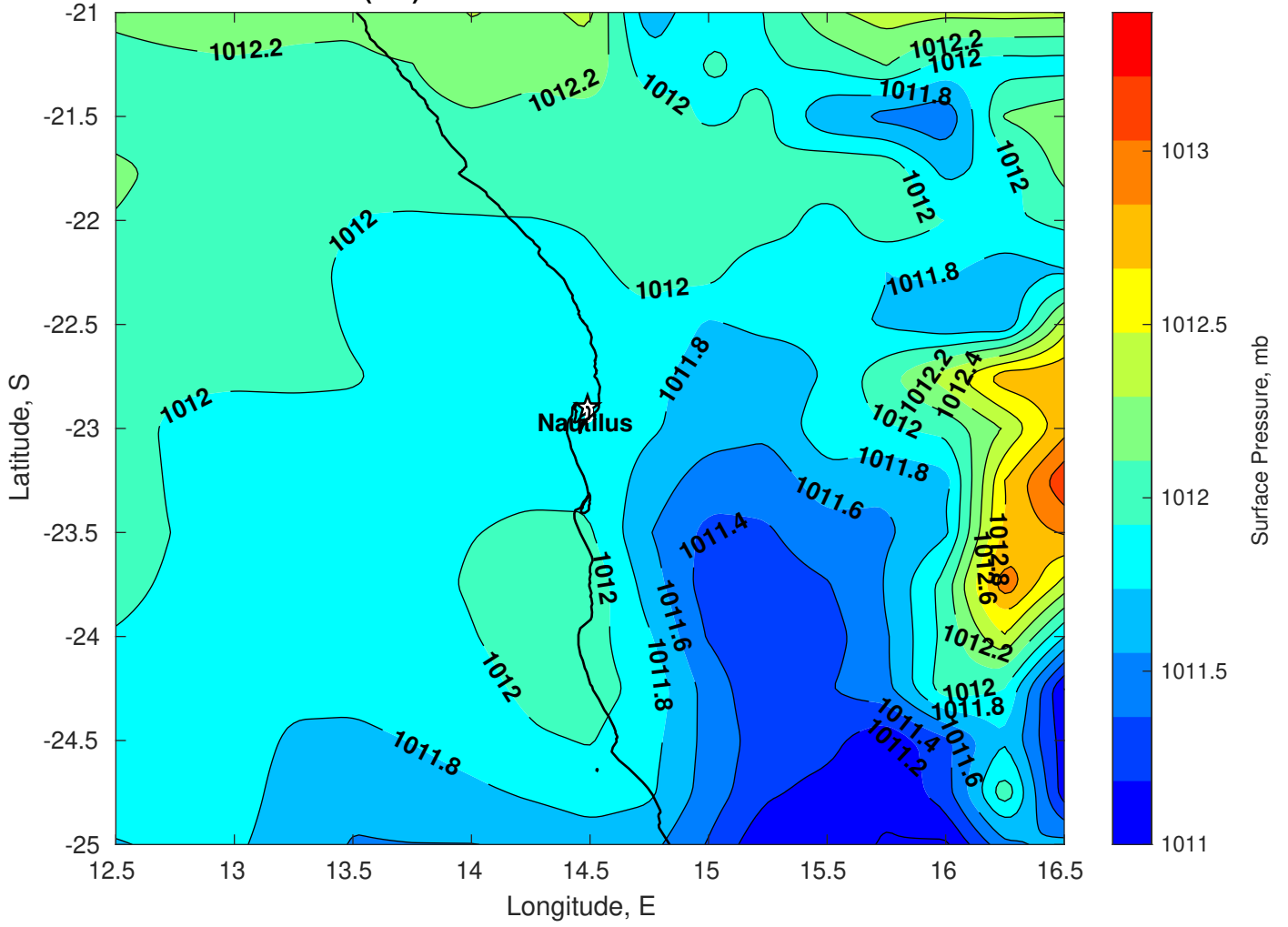
Surface Pressure (mb) for Nautilus at 14-Mar-2025 00:00:00
