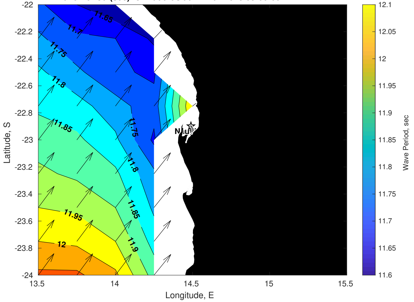
Wave Period (sec) for Nautilus at 12-Mar-2025 09:00:00
