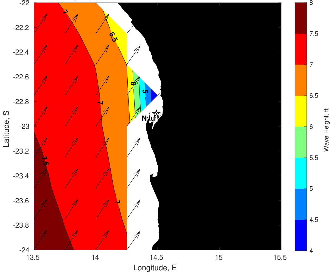
Wave Height (ft) for Nautilus at 12-Mar-2025 09:00:00
