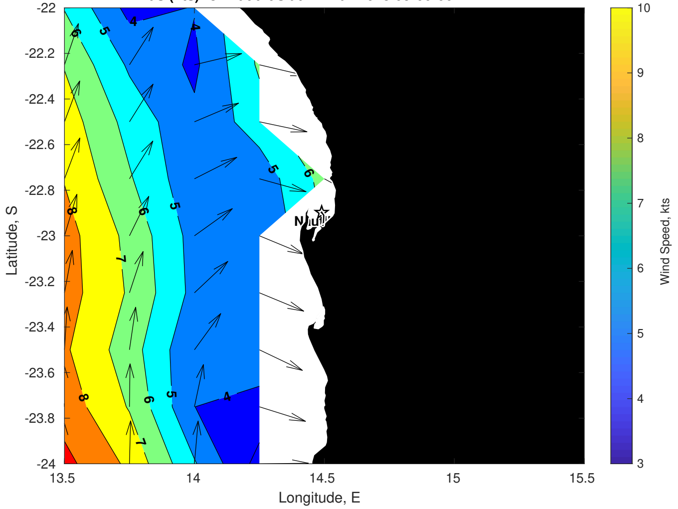
Winds (kts) for Nautilus at 12-Mar-2025 09:00:00
