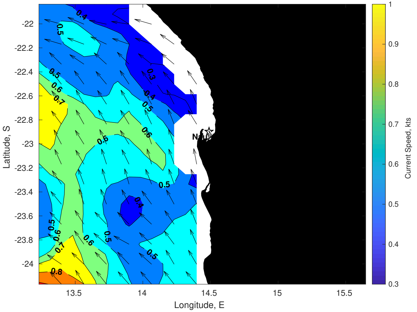
Surface Currents for Nautilus at 11-Mar-2025 00:00:00
