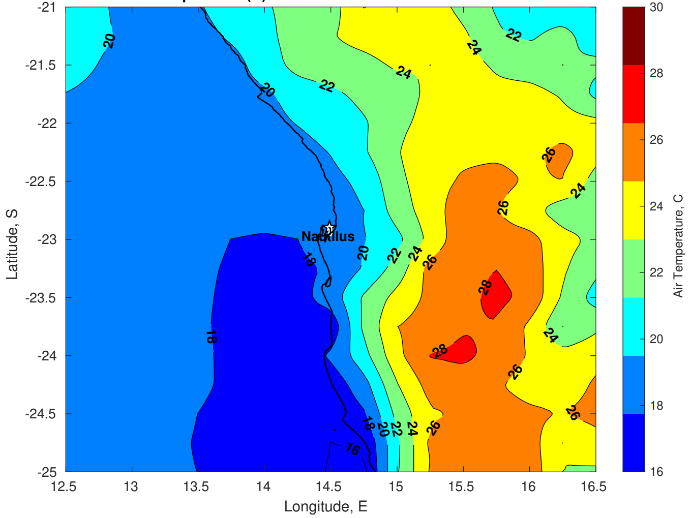
Air Temperature (C) for Nautilus at 12-Mar-2025
