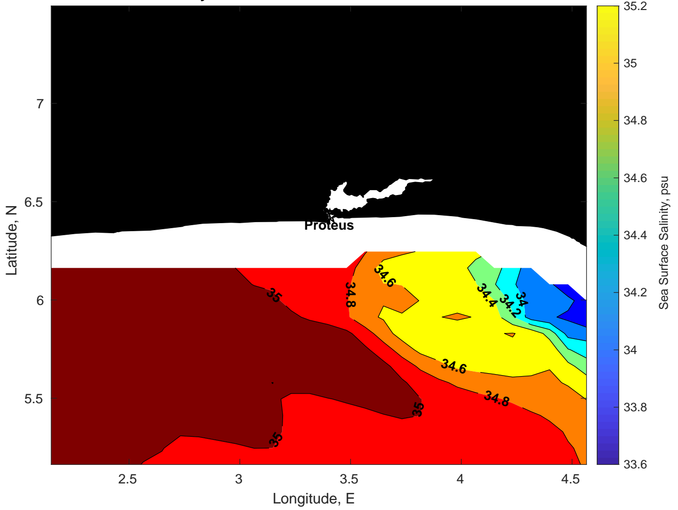
Surface Salinity for Proteus at 11-Mar-2025 00:00:00
