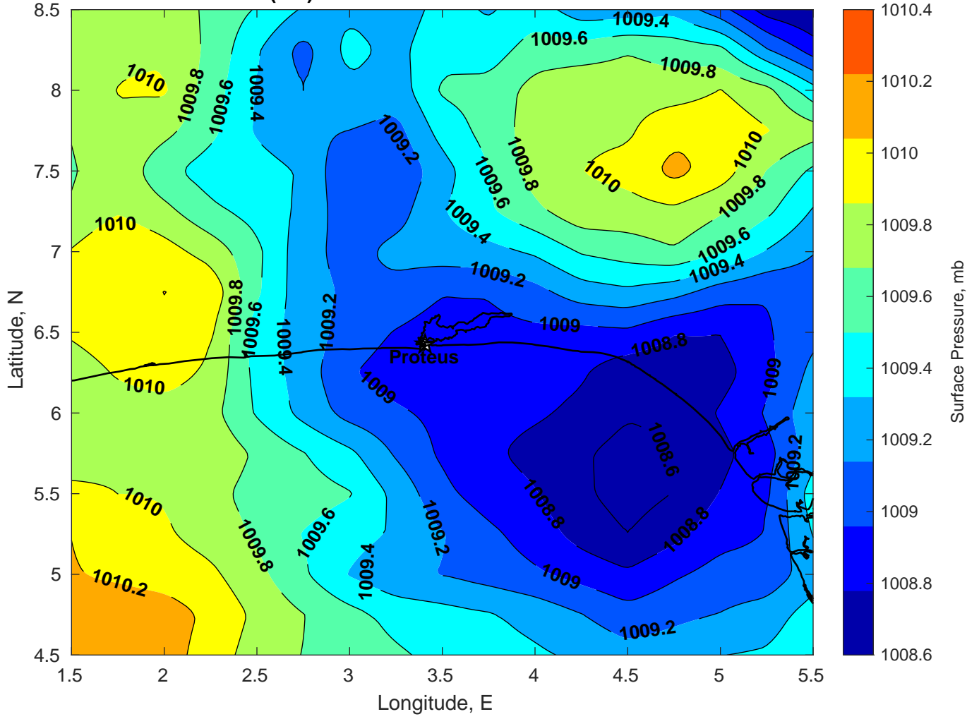
Surface Pressure (mb) for Proteus at 12-Mar-2025 00:00:00
