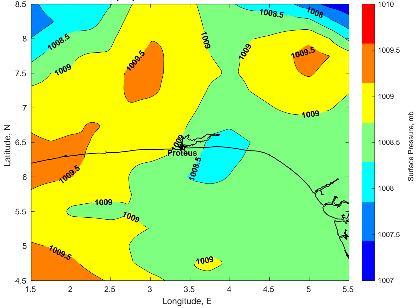
Surface Pressure (mb) for Proteus at 13-Mar-2025 00:00:00
