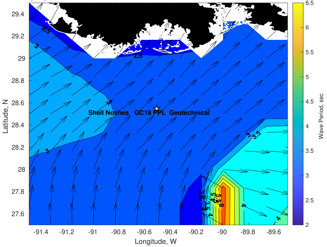
Wave Period (sec) for Shell Noches GC19 PPL Geotechnical at 12-Mar-2025 09:00:00
