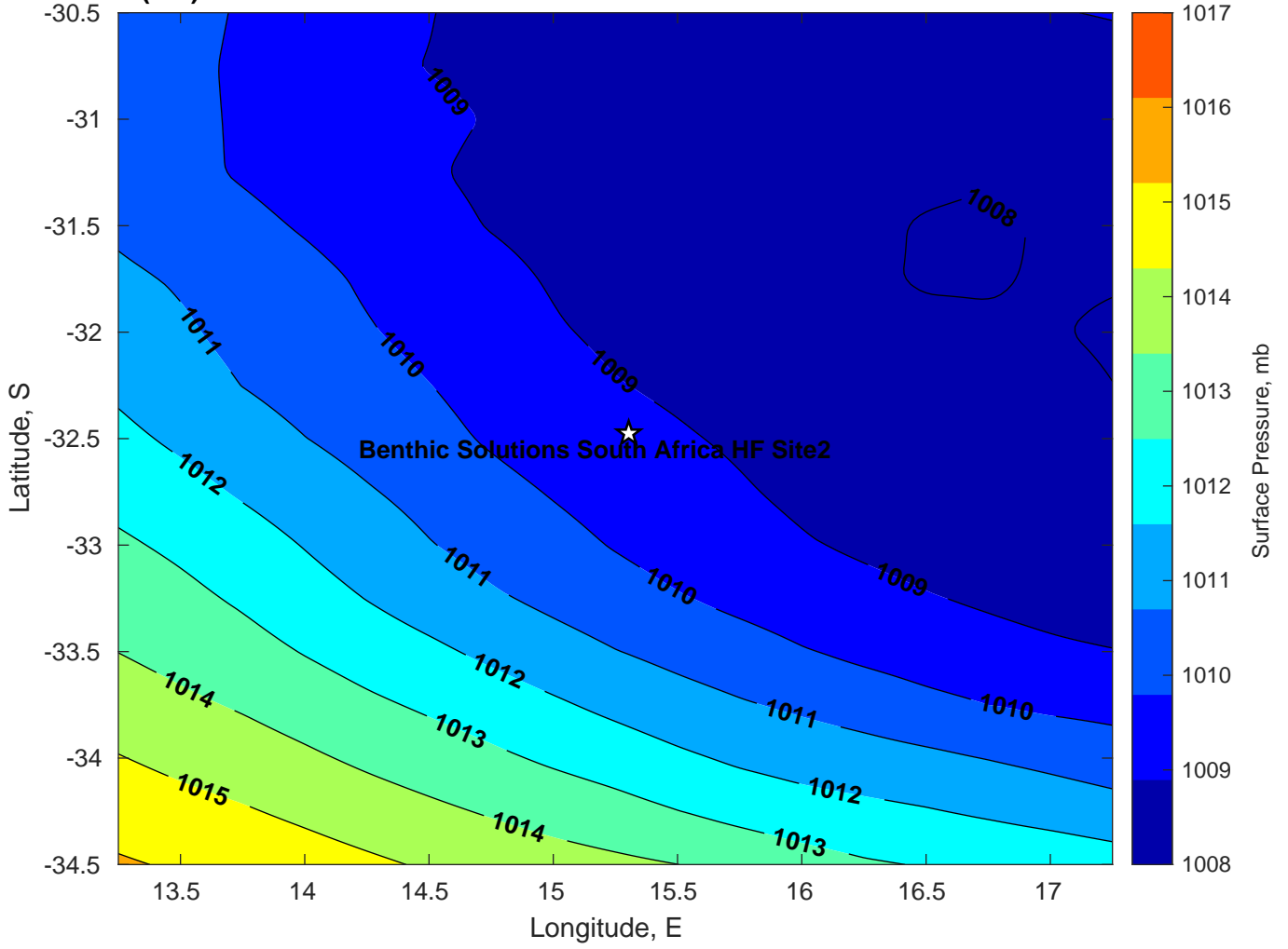
Surface Pressure (mb) for Benthic Solutions South Africa HF Site2 at 14-Mar-2025 00:00:00
