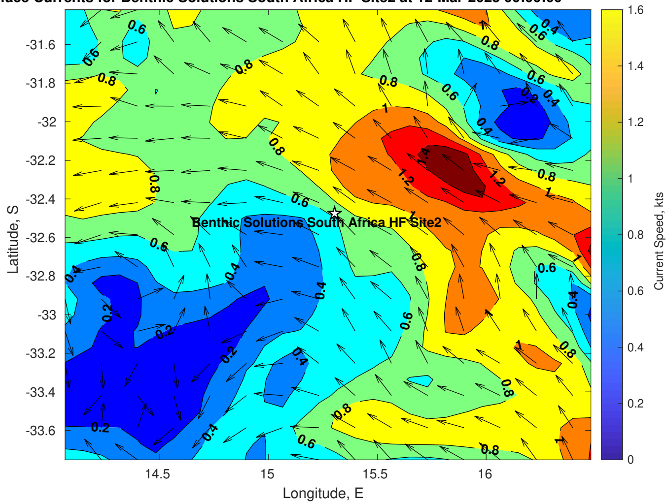
Surface Currents for Benthic Solutions South Africa HF Site2 at 12-Mar-2025 00:00:00
