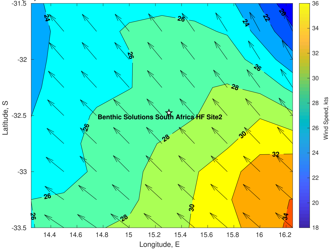
Winds (kts) for Benthic Solutions South Africa HF Site2 at 13-Mar-2025 09:00:00
