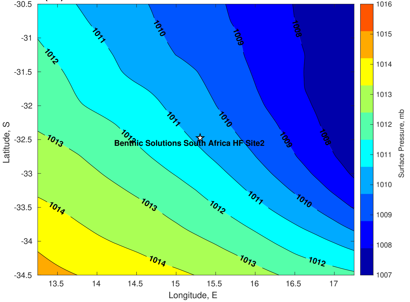
Surface Pressure (mb) for Benthic Solutions South Africa HF Site2 at 13-Mar-2025 00:00:00
