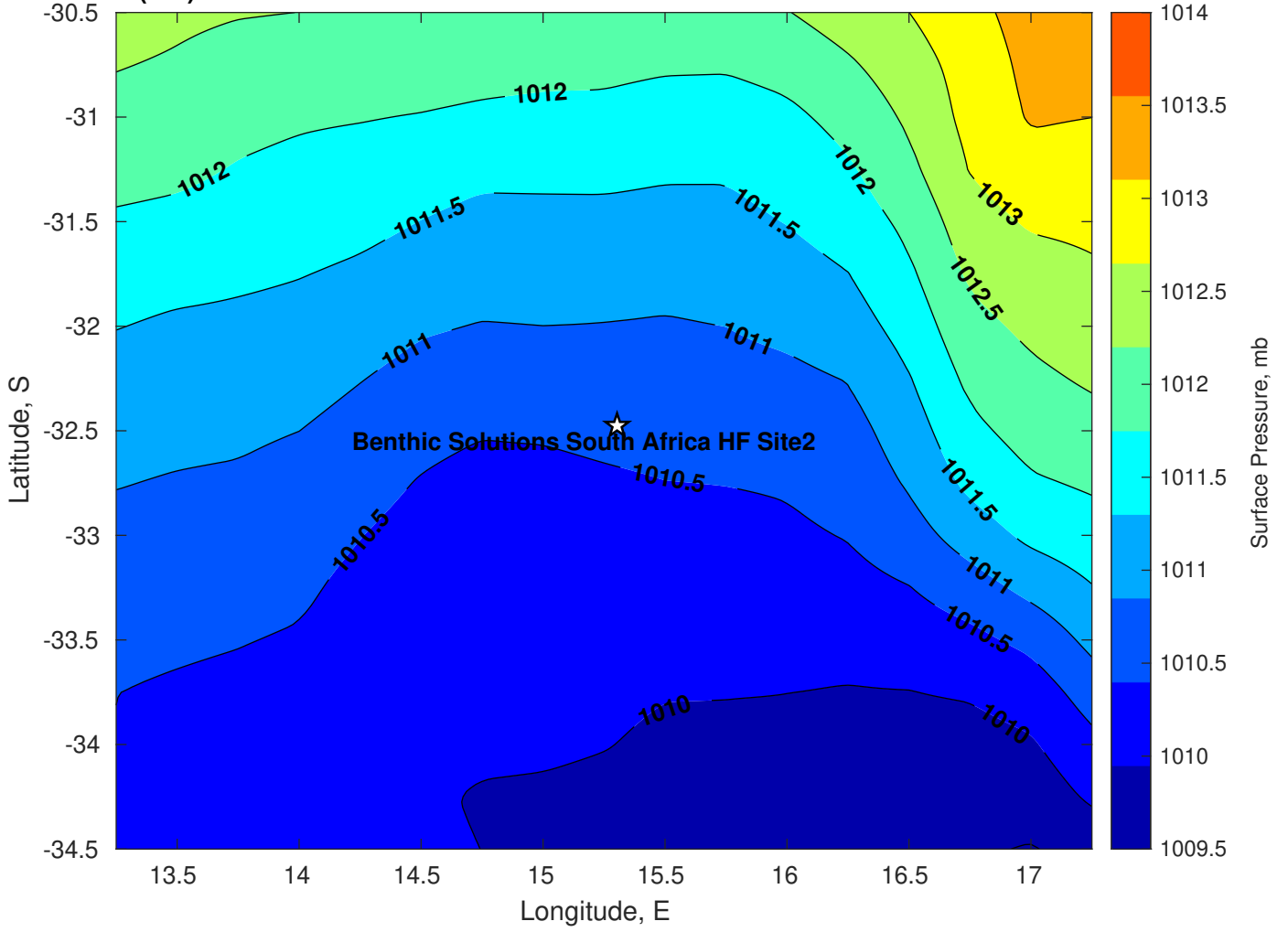
Surface Pressure (mb) for Benthic Solutions South Africa HF Site2 at 15-Mar-2025 00:00:00
