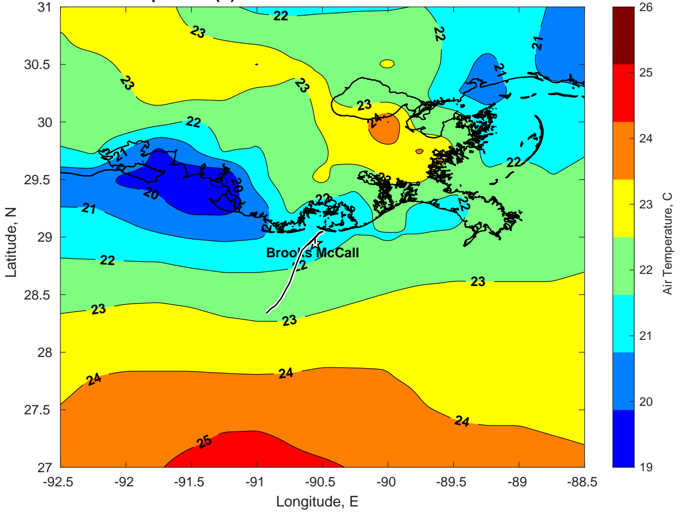
Air Temperature (C) for Brooks McCall at 13-Mar-2025
