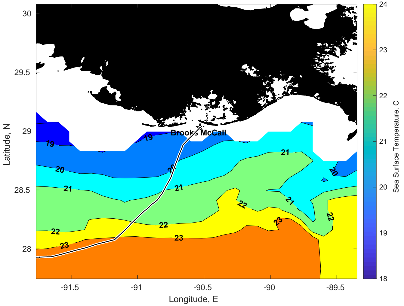
SST for Brooks McCall at 12-Mar-2025 00:00:00
