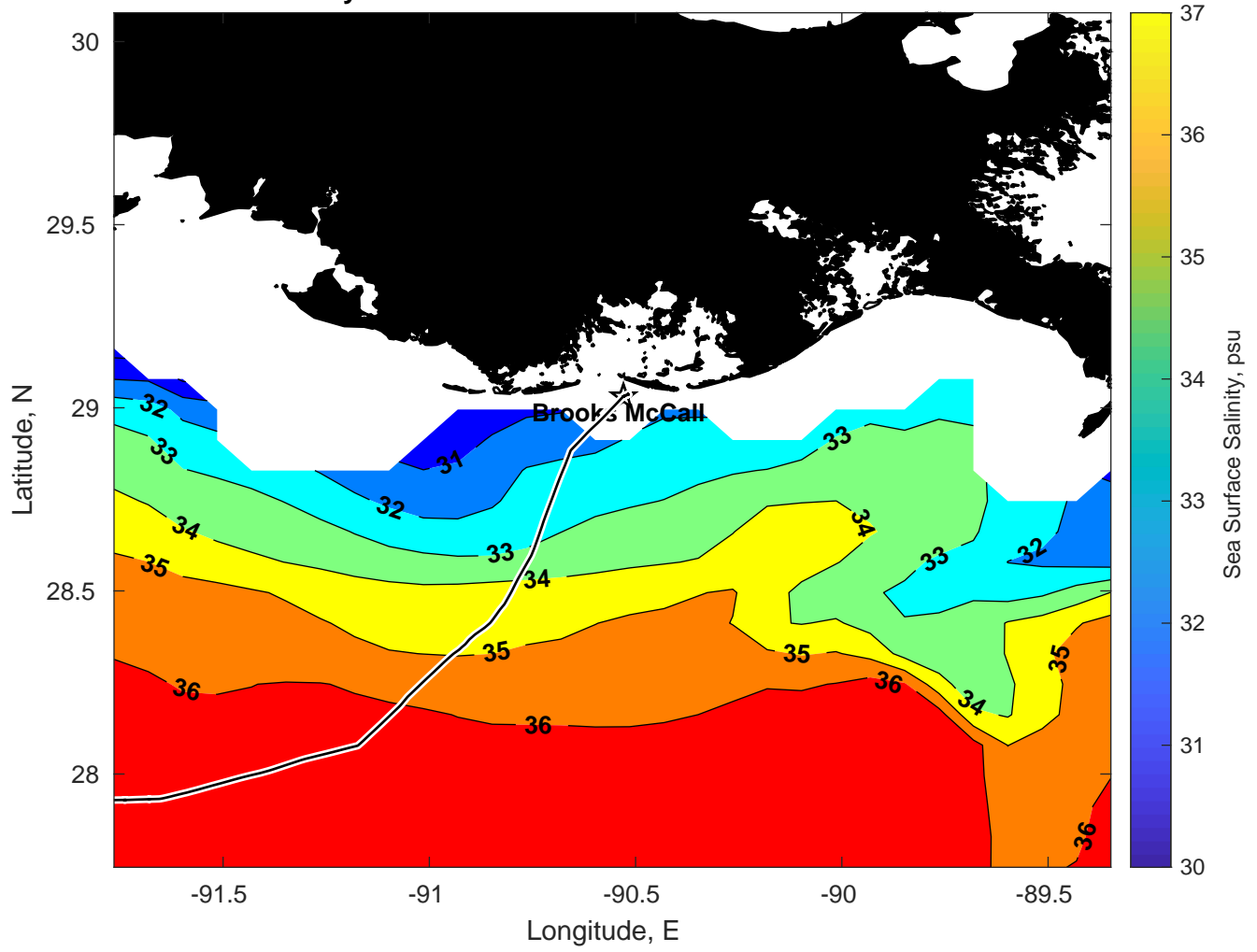
Surface Salinity for Brooks McCall at 12-Mar-2025 00:00:00
