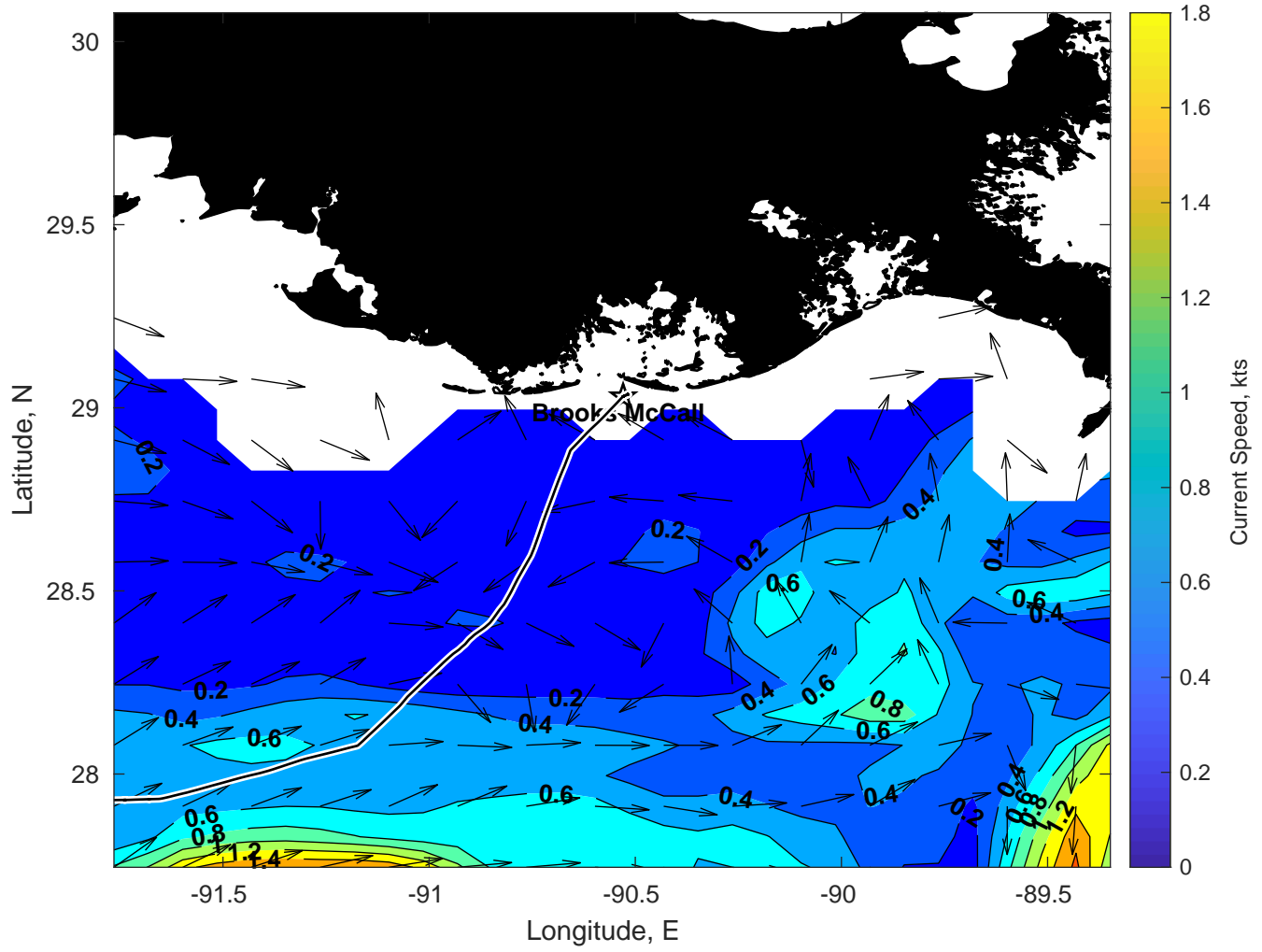
Surface Currents for Brooks McCall at 12-Mar-2025 00:00:00
