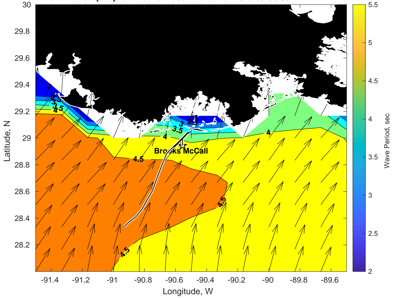
Wave Period (sec) for Brooks McCall at 13-Mar-2025 09:00:00
