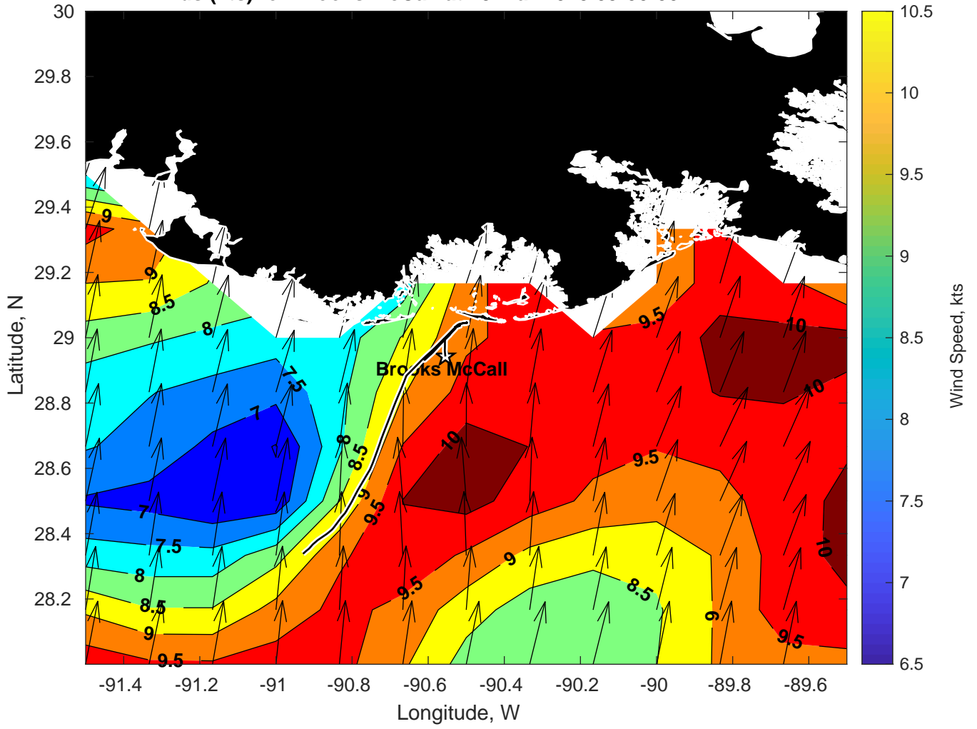
Winds (kts) for Brooks McCall at 13-Mar-2025 09:00:00
