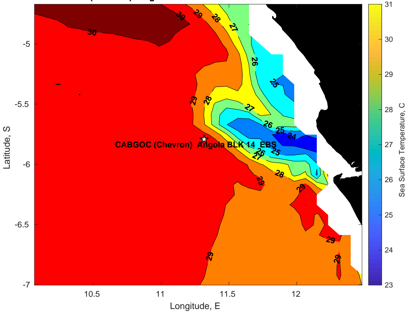
SST for CABGOC (Chevron) Angola BLK 14 EBS at 12-Mar-2025 00:00:00
