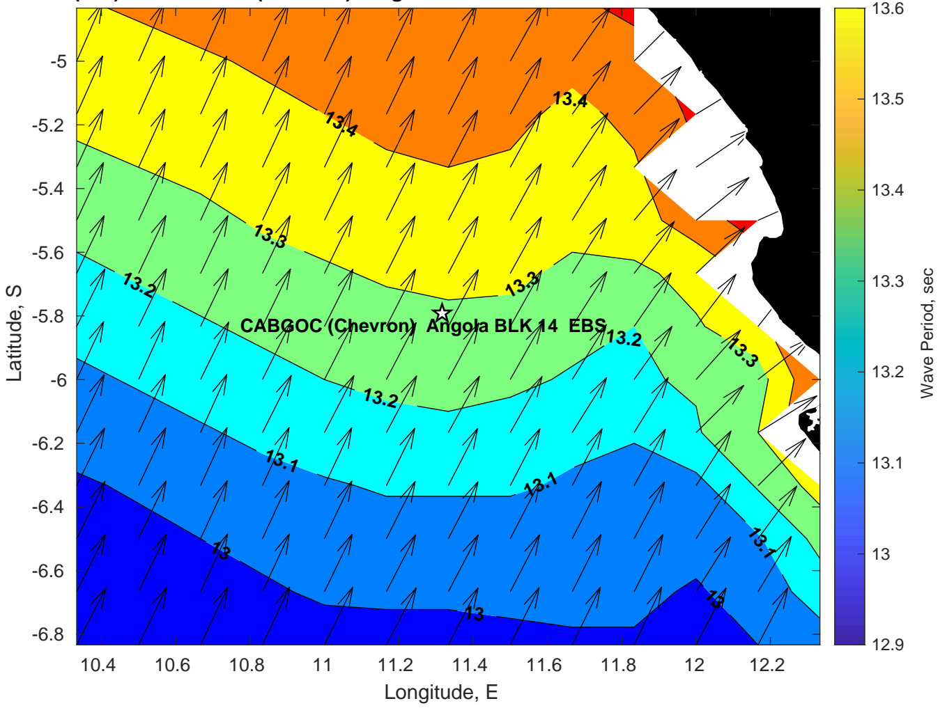
Wave Period (sec) for CABGOC (Chevron) Angola BLK 14 EBS at 13-Mar-2025 09:00:00
