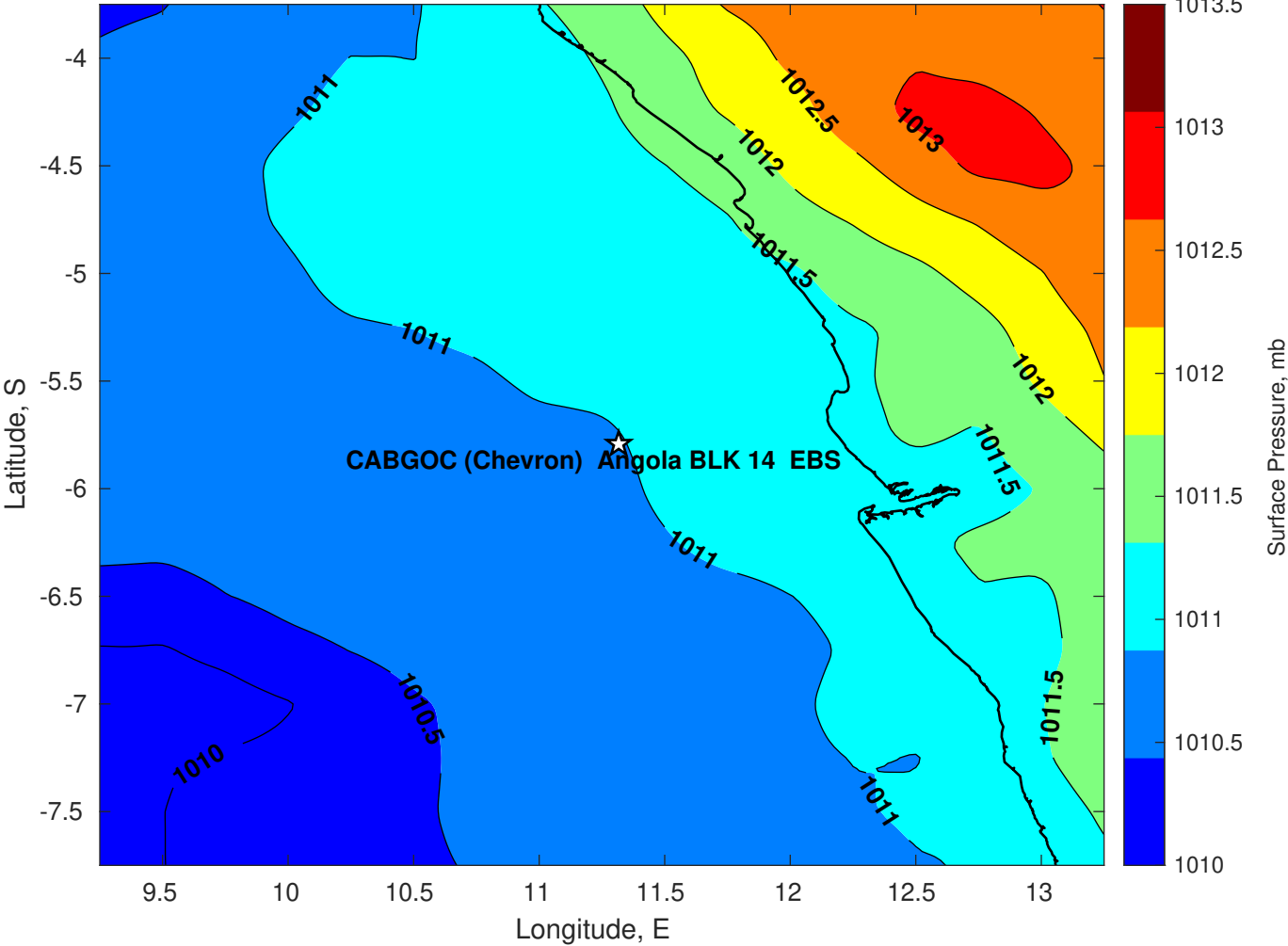
Surface Pressure (mb) for CABGOC (Chevron) Angola BLK 14 EBS at 14-Mar-2025 00:00:00
