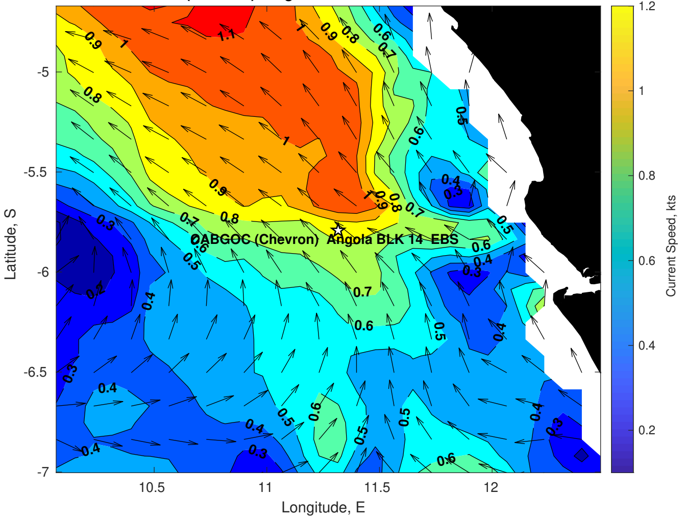
Surface Currents for CABGOC (Chevron) Angola BLK 14 EBS at 12-Mar-2025 00:00:00
