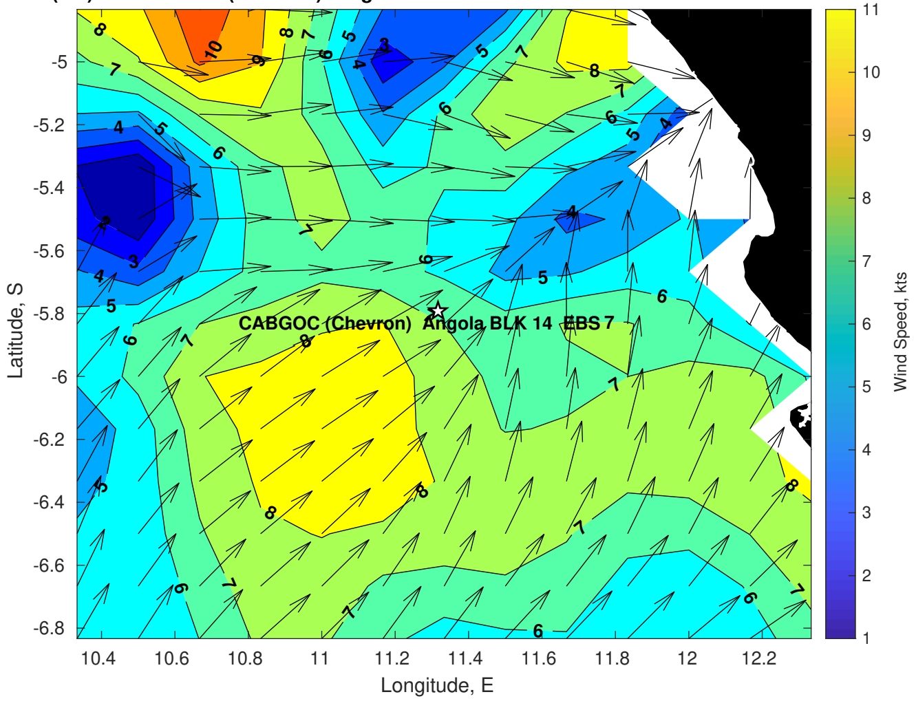
Winds (kts) for CABGOC (Chevron) Angola BLK 14 EBS at 13-Mar-2025 09:00:00
