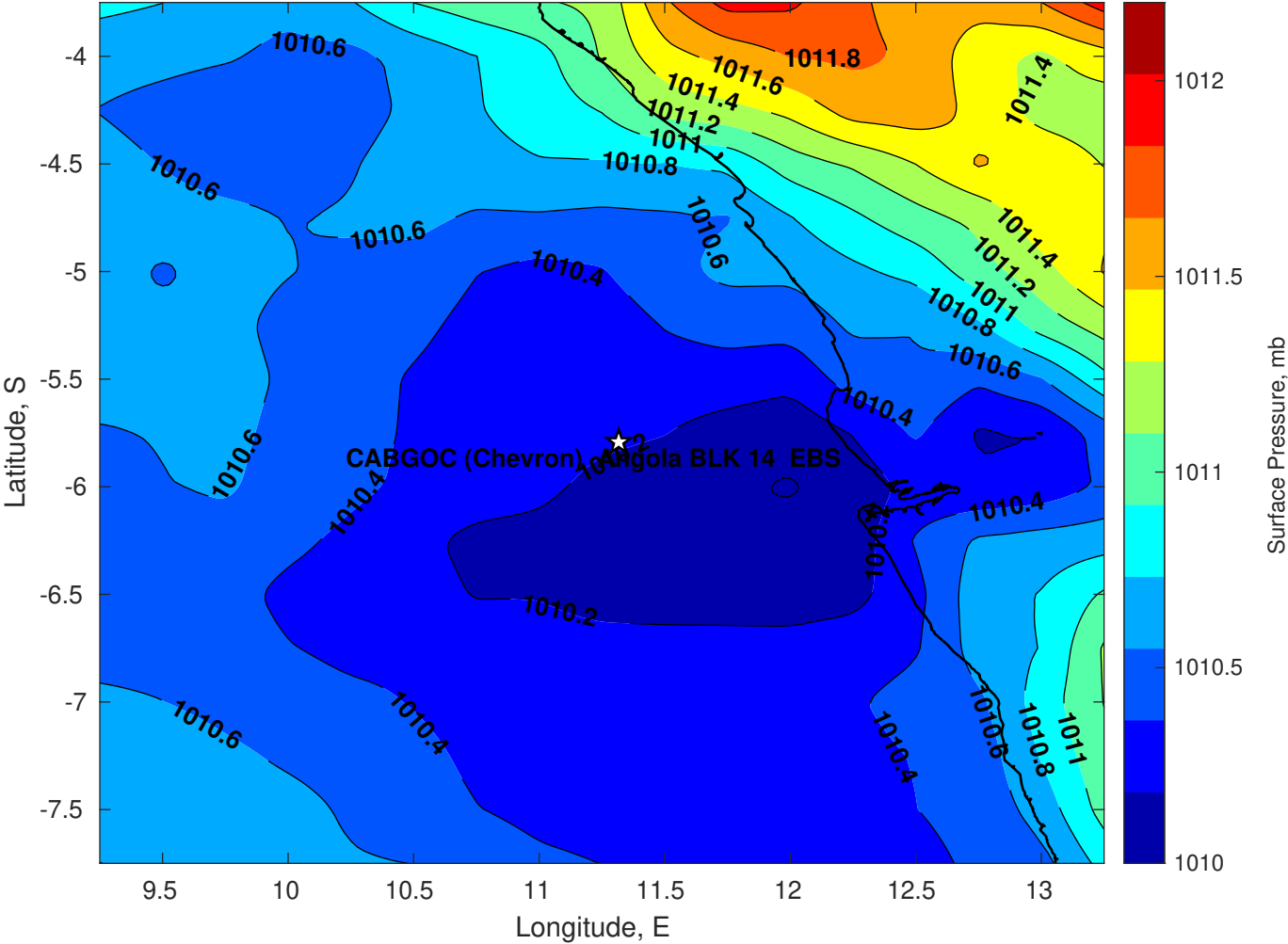
Surface Pressure (mb) for CABGOC (Chevron) Angola BLK 14 EBS at 15-Mar-2025 00:00:00
