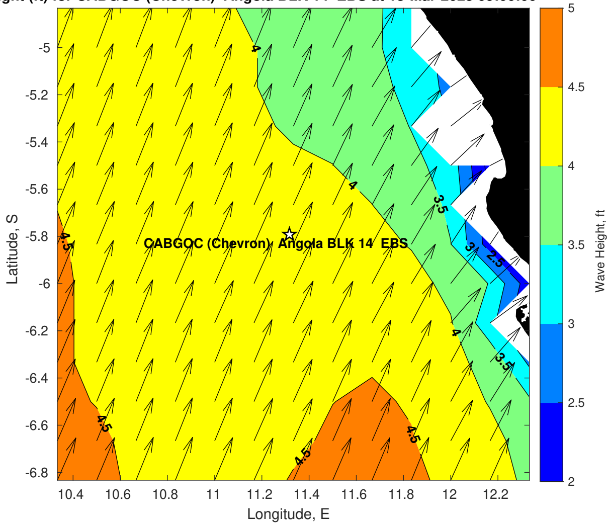
Wave Height (ft) for CABGOC (Chevron) Angola BLK 14 EBS at 13-Mar-2025 09:00:00
