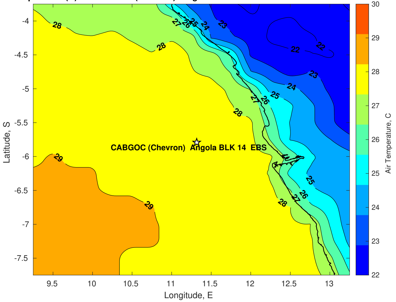
Air Temperature (C) for CABGOC (Chevron) Angola BLK 14 EBS at 13-Mar-2025
