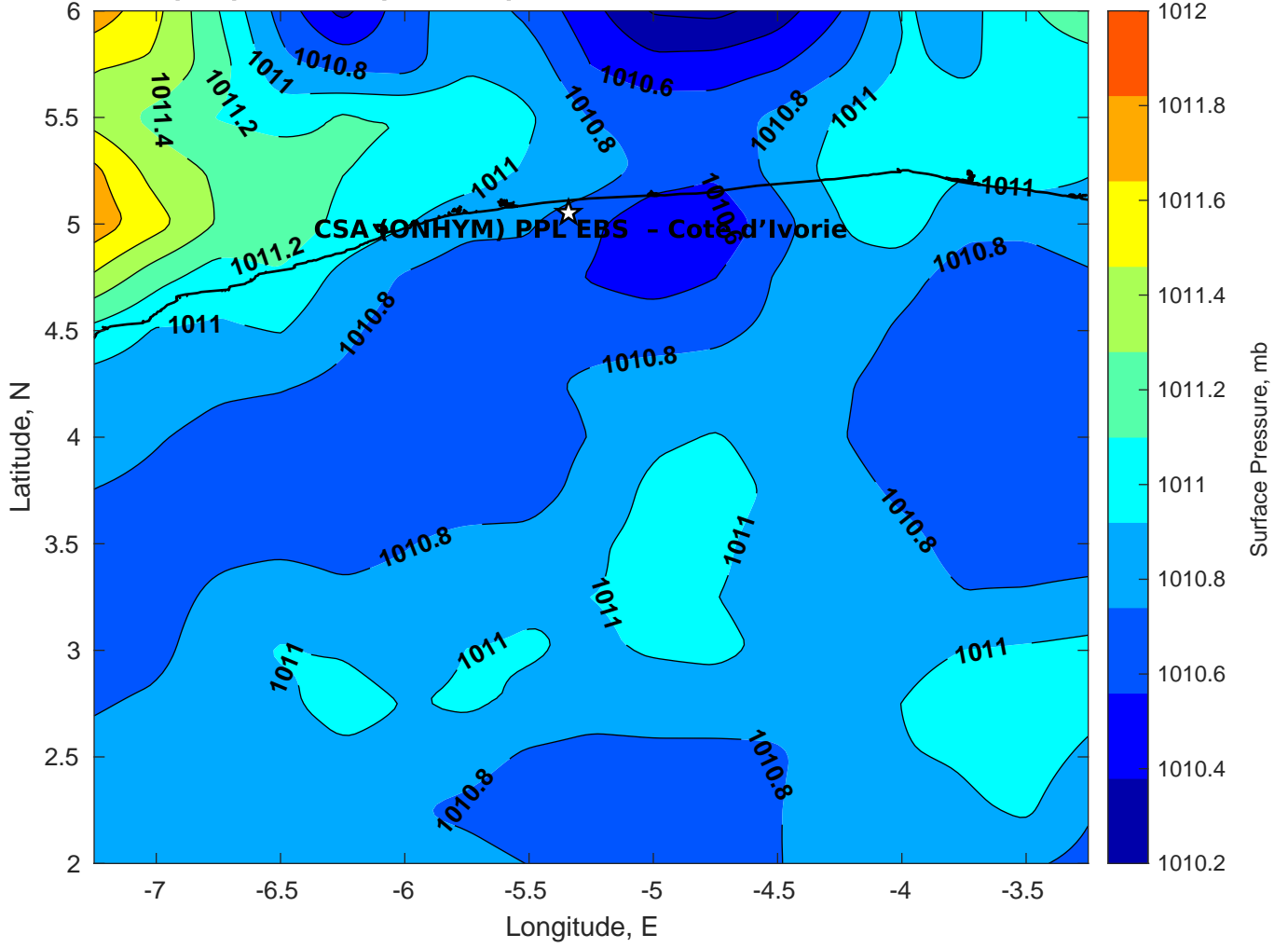
Surface Pressure (mb) for CSA (ONHYM) PPL EBS - Cote d'Ivoire at 14-Mar-2025 00:00:00
