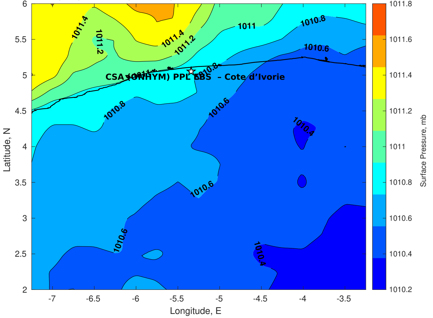
Surface Pressure (mb) for CSA (ONHYM) PPL EBS - Cote d'Ivoire at 15-Mar-2025 00:00:00
