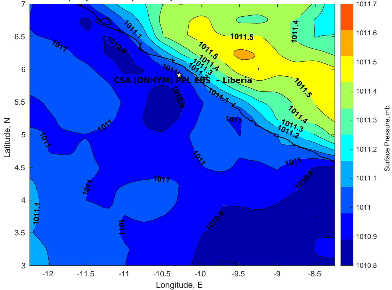
Surface Pressure (mb) for CSA (ONHYM) PPL EBS - Liberia at 15-Mar-2025 00:00:00
