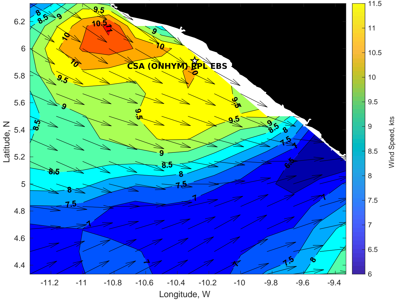
Winds (kts) for CSA (ONHYM) PPL EBS - Liberia at 13-Mar-2025 09:00:00
