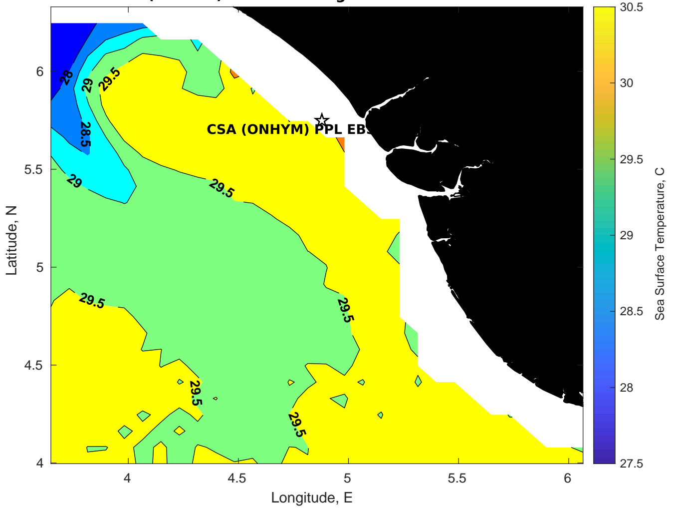
SST for CSA (ONHYM) PPL EBS - Nigeria at 12-Mar-2025 00:00:00
