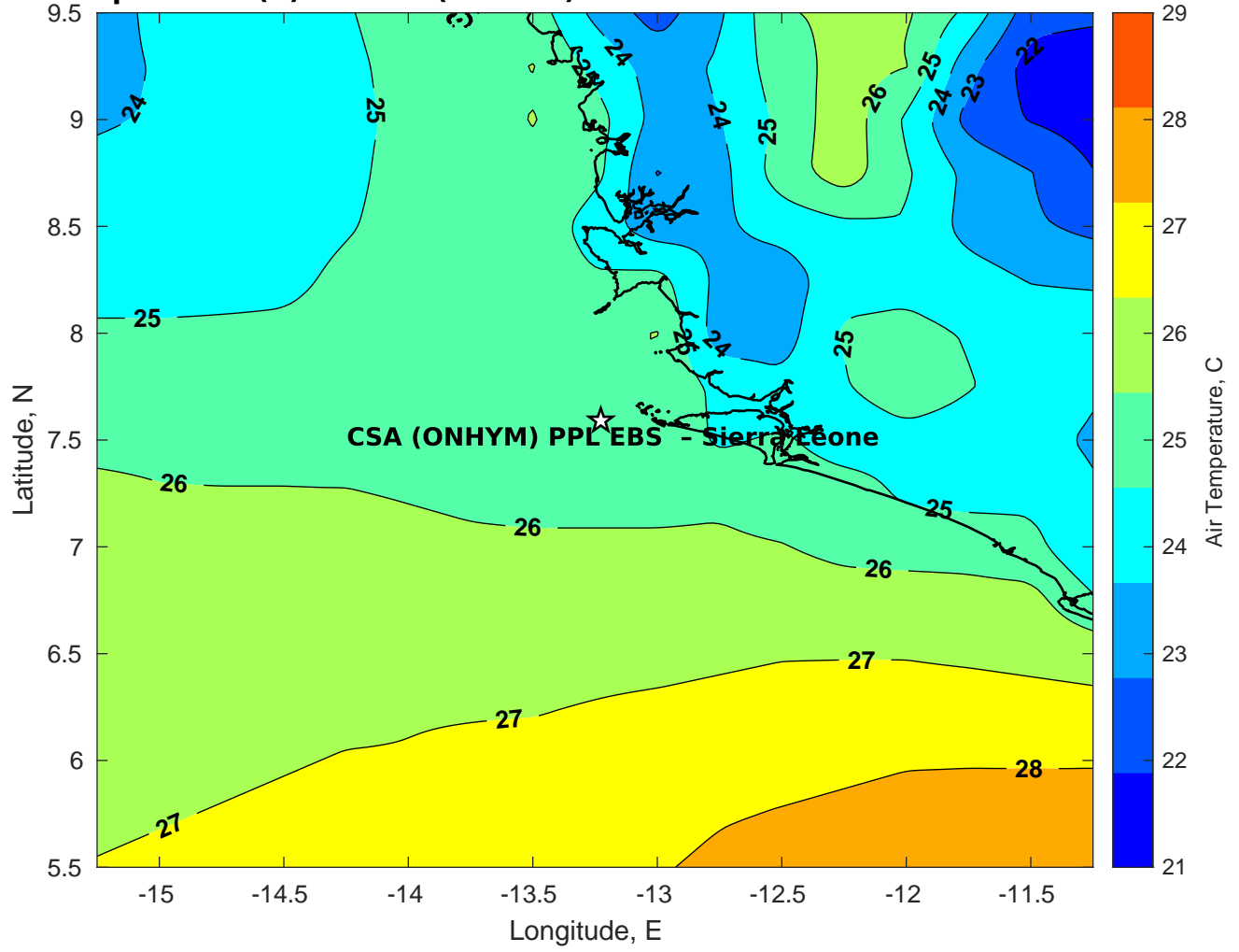
Air Temperature (C) for CSA (ONHYM) PPL EBS - Sierra Leone at 13-Mar-2025
