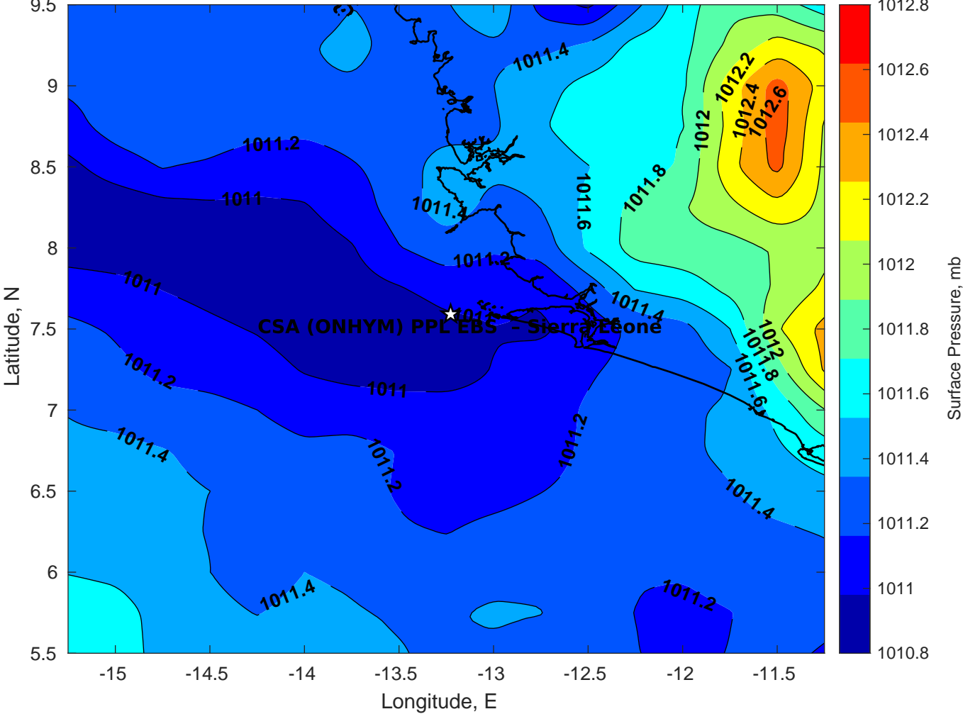
Surface Pressure (mb) for CSA (ONHYM) PPL EBS - Sierra Leone at 14-Mar-2025 00:00:00
